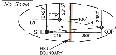
Detail "A" No Scale
