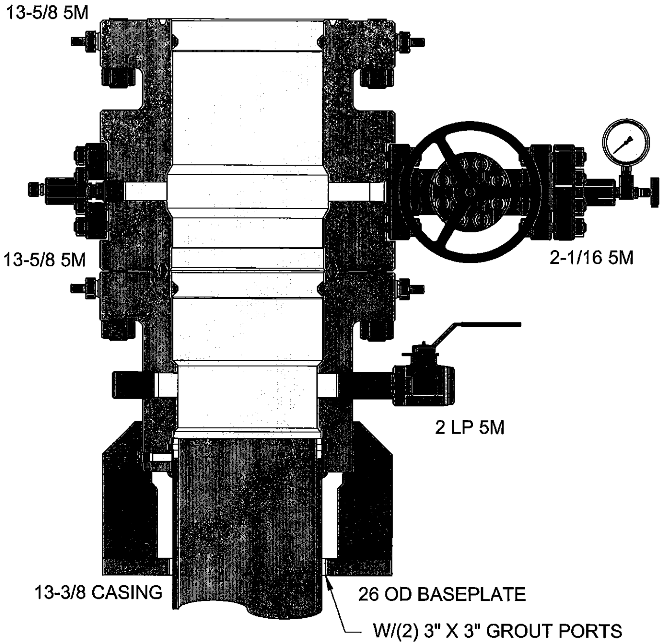
FIGURE 1 – LANDING MULTI-BOWL
