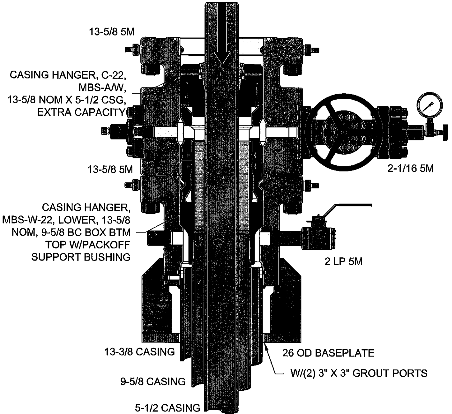
FIGURE 4 – HANGER INSTALLED
