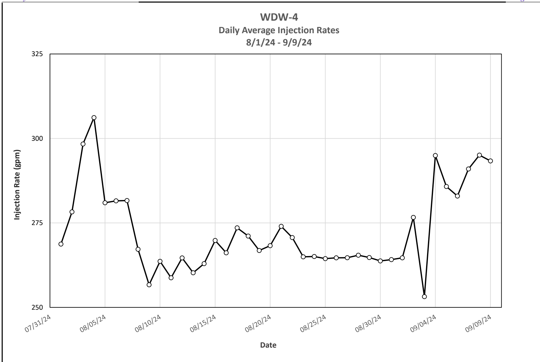
Figure 9 Daily Average Injection Rates 2024 Well Testing
