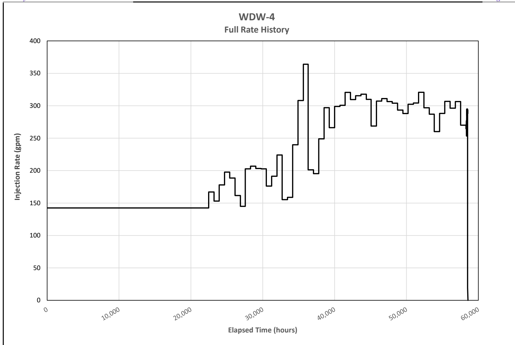
Figure 5 Full Rate History 2024 Well Testing
