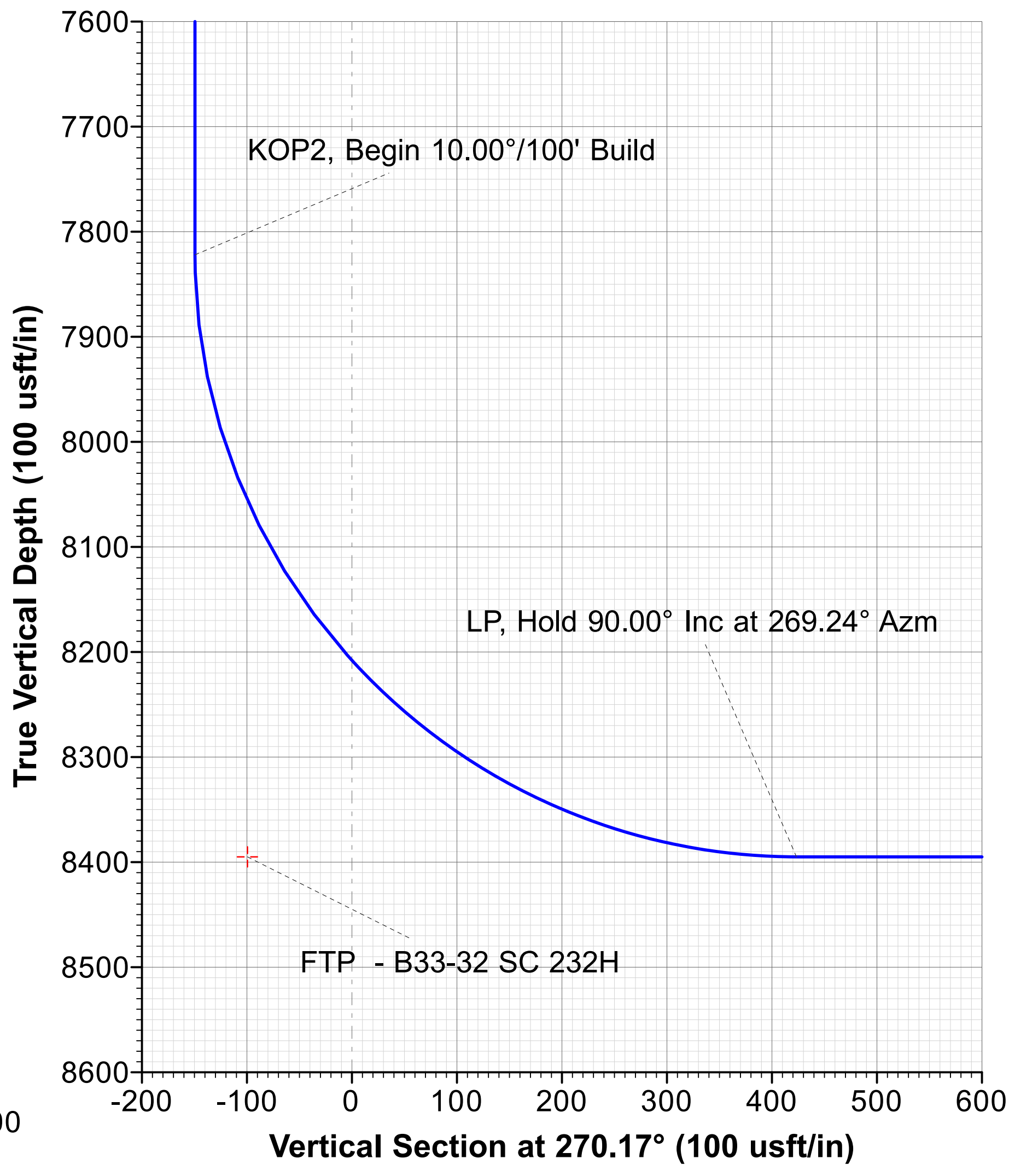
Vertical Section at 270.17° (100 usft/in)
