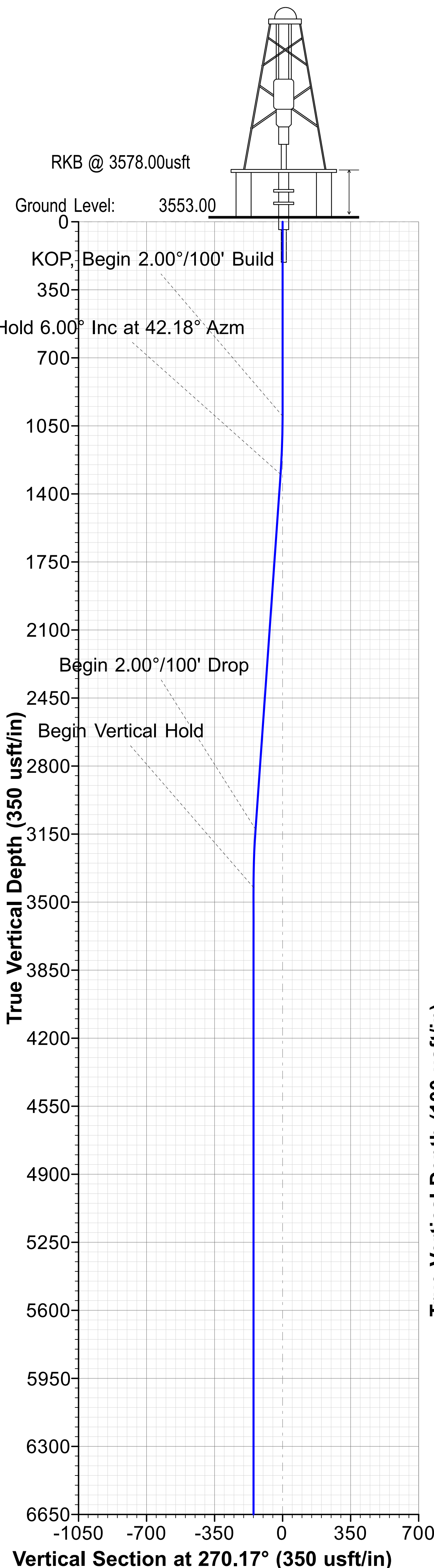
Vertical Section at 270.17° (350 usft/in)
