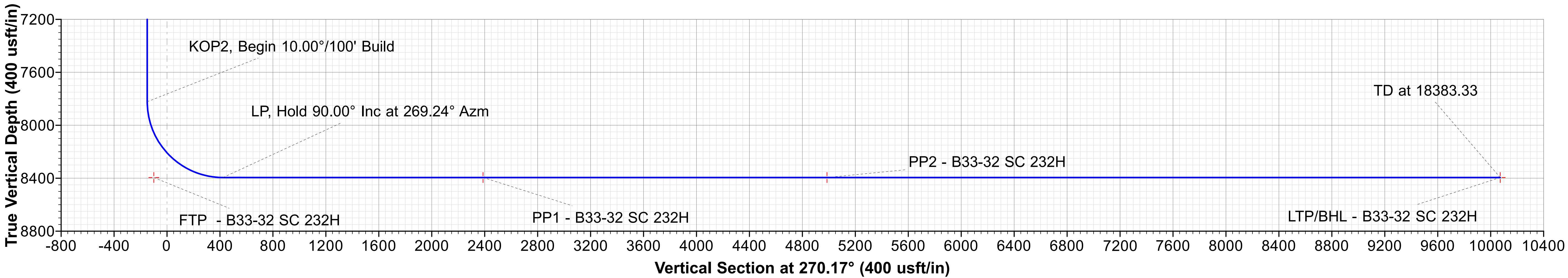
Vertical Section at 270.17° (400 usft/in)
