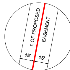
TYPICAL RIGHT-OF-WAY EASEMENT
