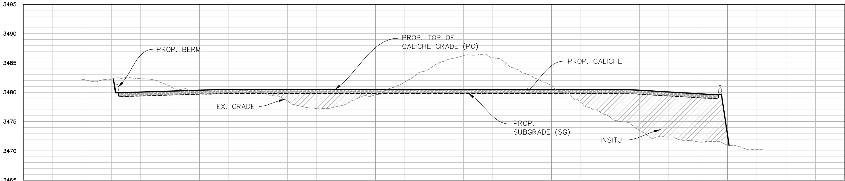
CROSS SECTION "A" H: 1" = 150' V: 1" = 15'
