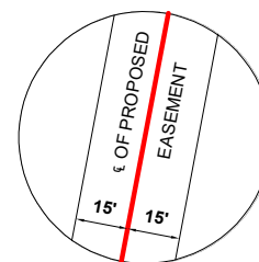
TYPICAL RIGHT-OF-WAY EASEMENT (L1, L2, L7 & L8)
