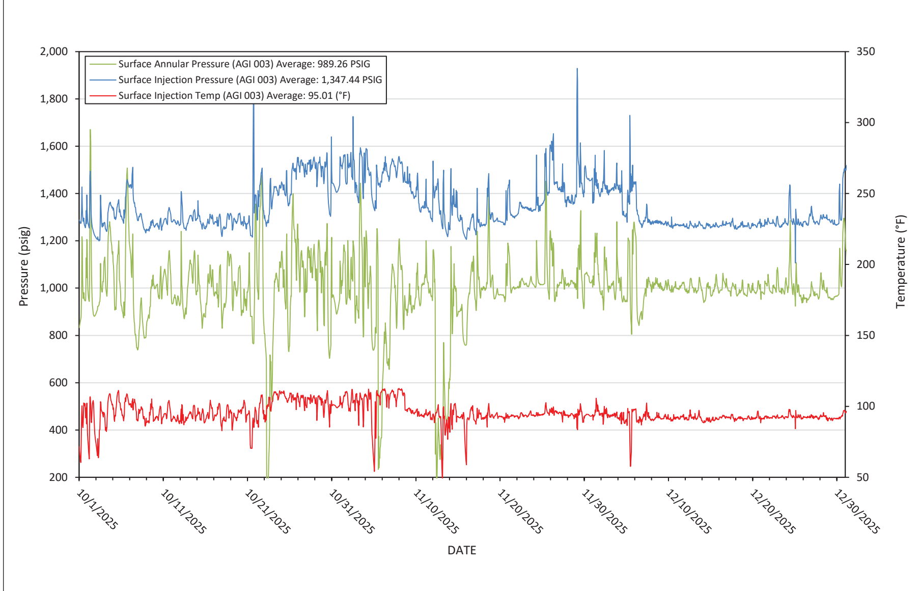
FIGURE 3. SALT CREEK AGI #003 SURFACE INJECTION PRESSURE, ANNULAR PRESSURE AND INJECTION TEMPERATURE
