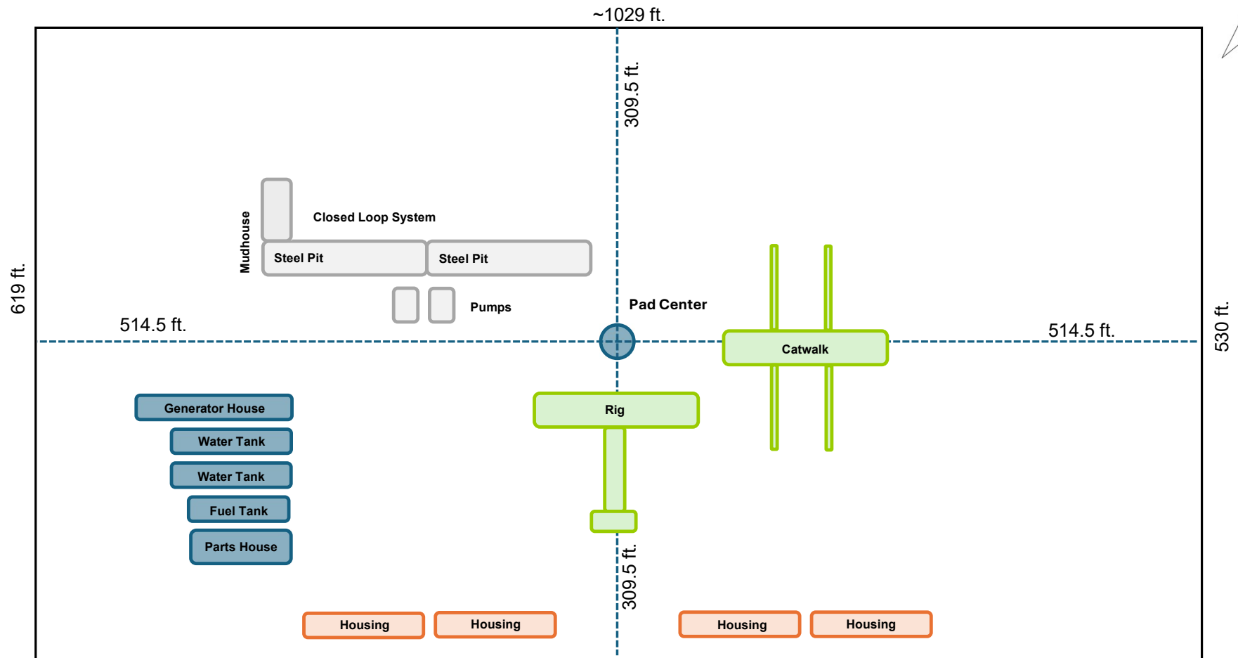
Boom Boom Pad (GTO Fed) Rig Layout
