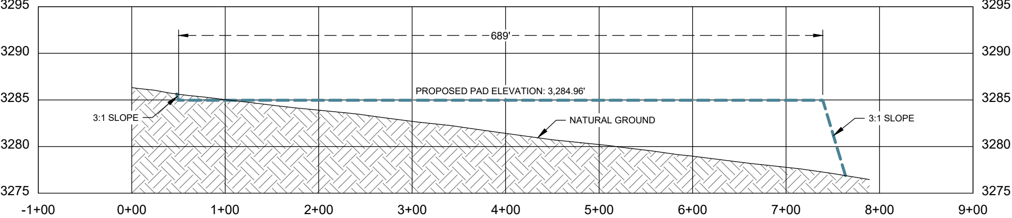
PROFILE VIEW: B - B'
