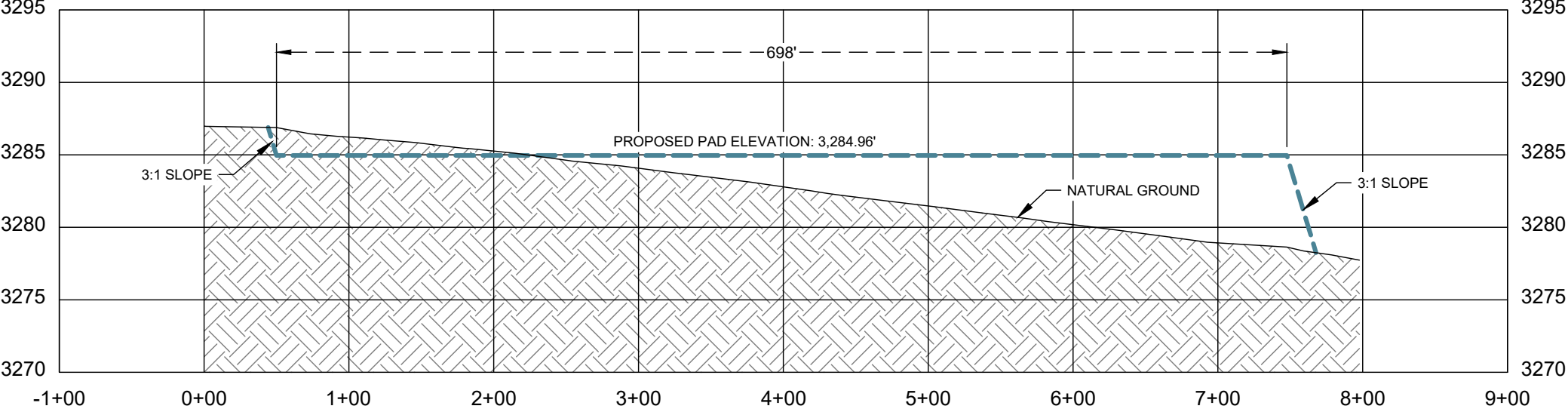
PROFILE VIEW: A - A'
