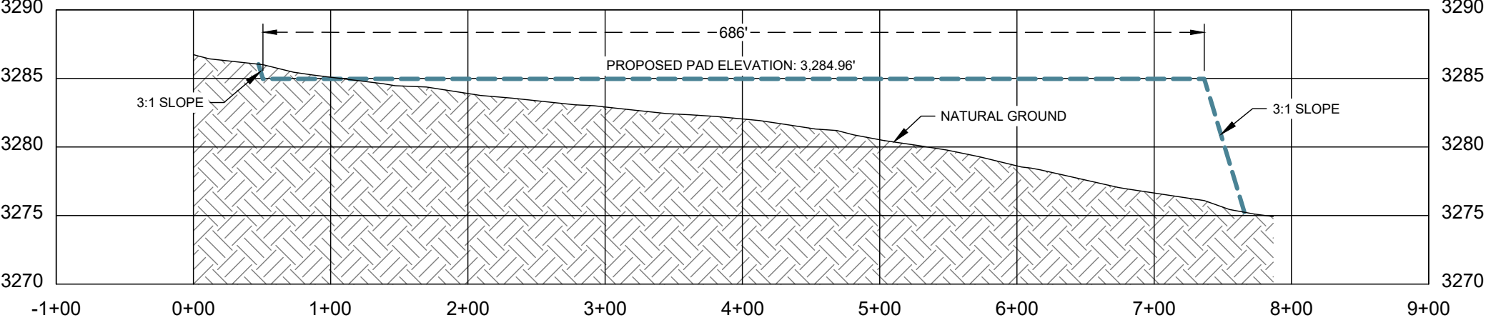
PROFILE VIEW: C - C'
