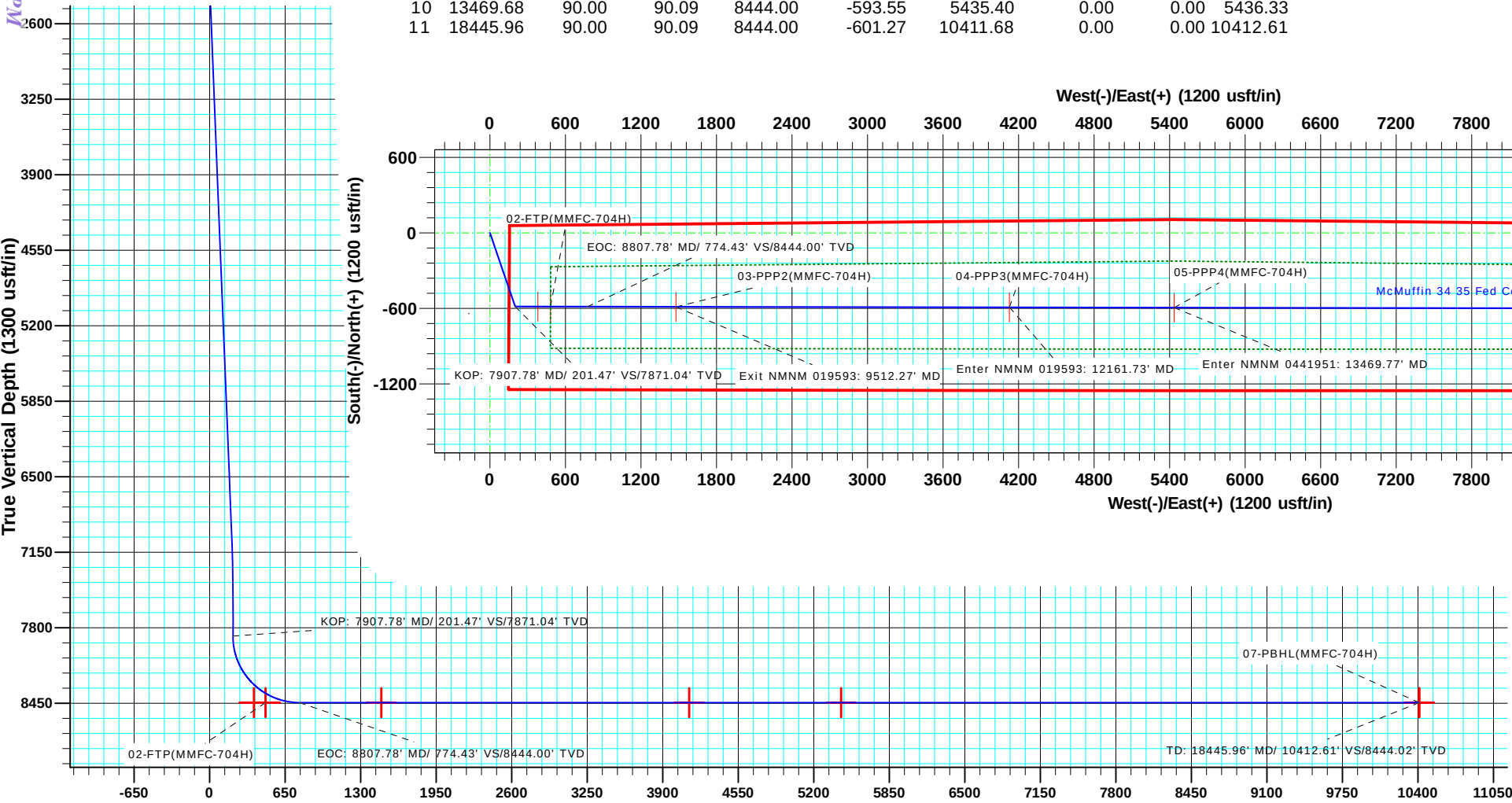
Vertical Section at 90.09° (1300 usft/in)
