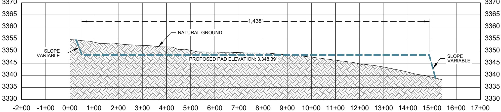
PROFILE VIEW: B - B'
