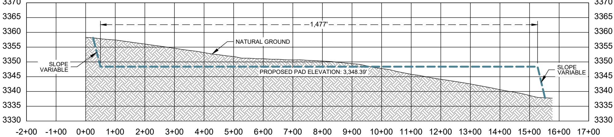
PROFILE VIEW: A - A'
