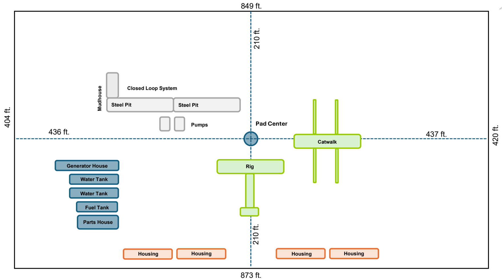
Asteroid West Pad Rig Layout
