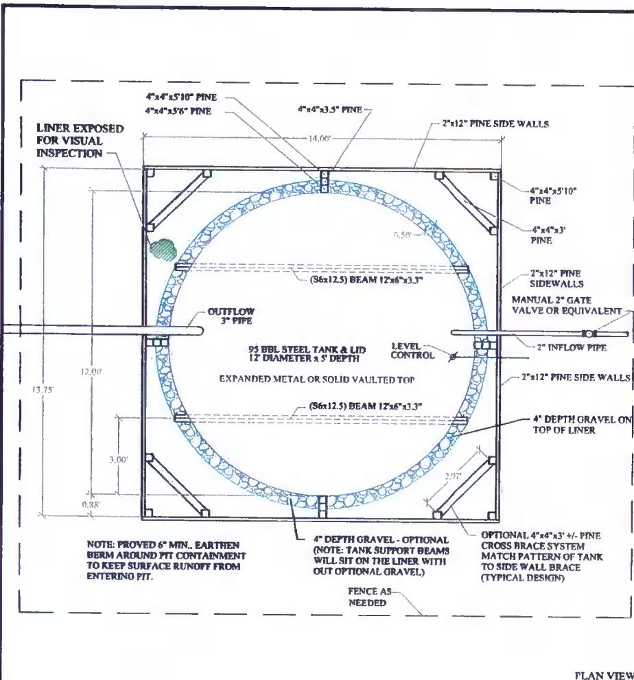
PLAN VIEW
