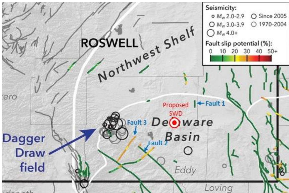
Figure 2. Modified Figure 3 from Snee and Zoback (2018). Map showing proposed location of Scrotch Owl 242128 Federal SWD #1 in relation to Snee and Zoback's results of their FSP analysis.
