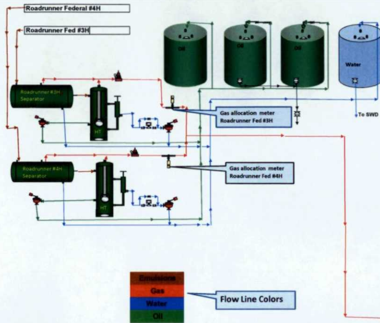
Roadrunner Federal #3H & #4H Tank Battery Sec 23, SENE, T23S-R30E
