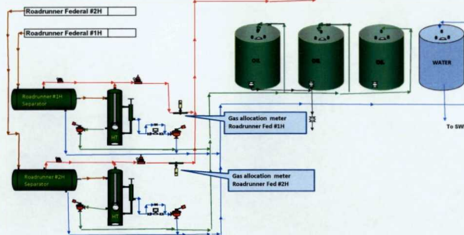
Roadrunner Federal #1H & #2H Tank Battery Sec 25, NWNW, T23S-R30E
