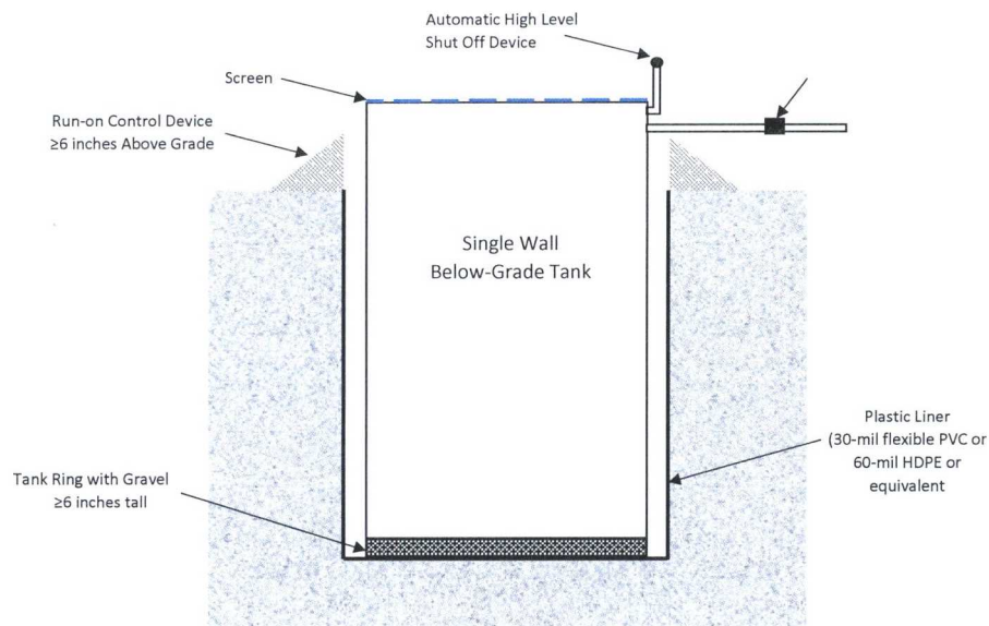
FIGURE 1. BGT DESIGN AND CONSTRUCTION – 19.15.17.11.1.(4)(a) NMAC
