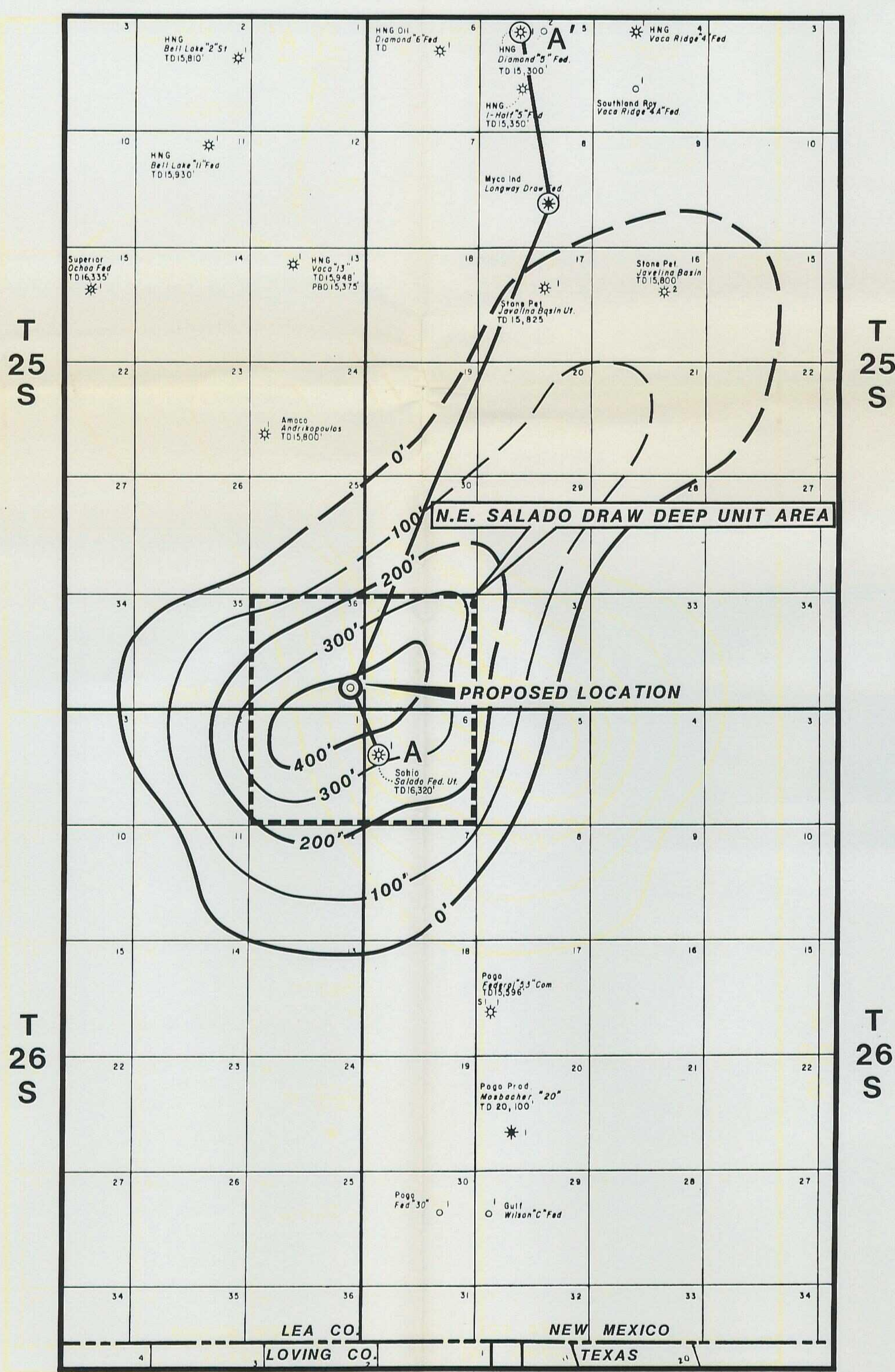
ISOPACH MAP UPPER MORROW SEDIMENTS SEISMICALLY DETERMINED ISOPACH
