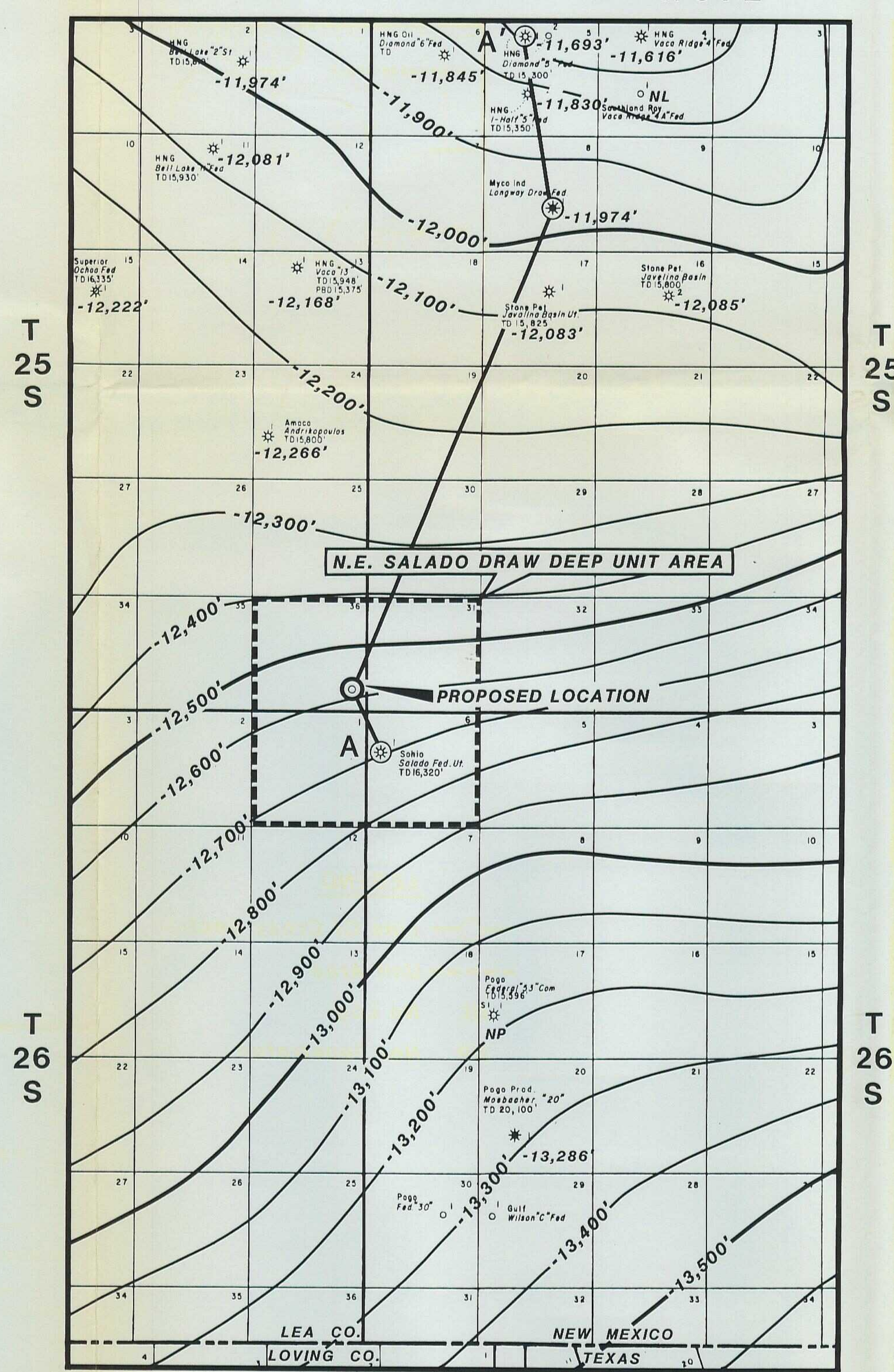
STRUCTURE MAP TOP MIDDLE MORROW SHALE
