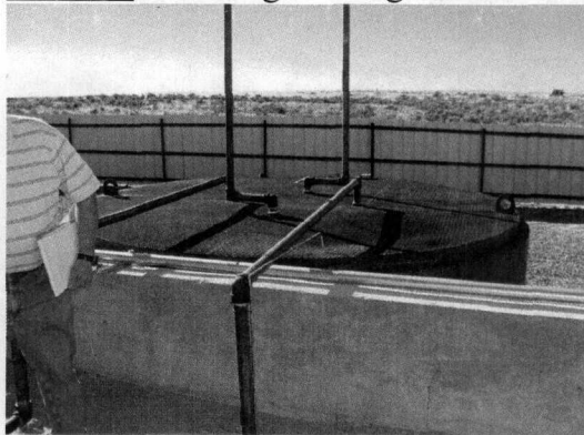
Photo 11: An engineered BGT used as an AST (leak detection) with no berms.
