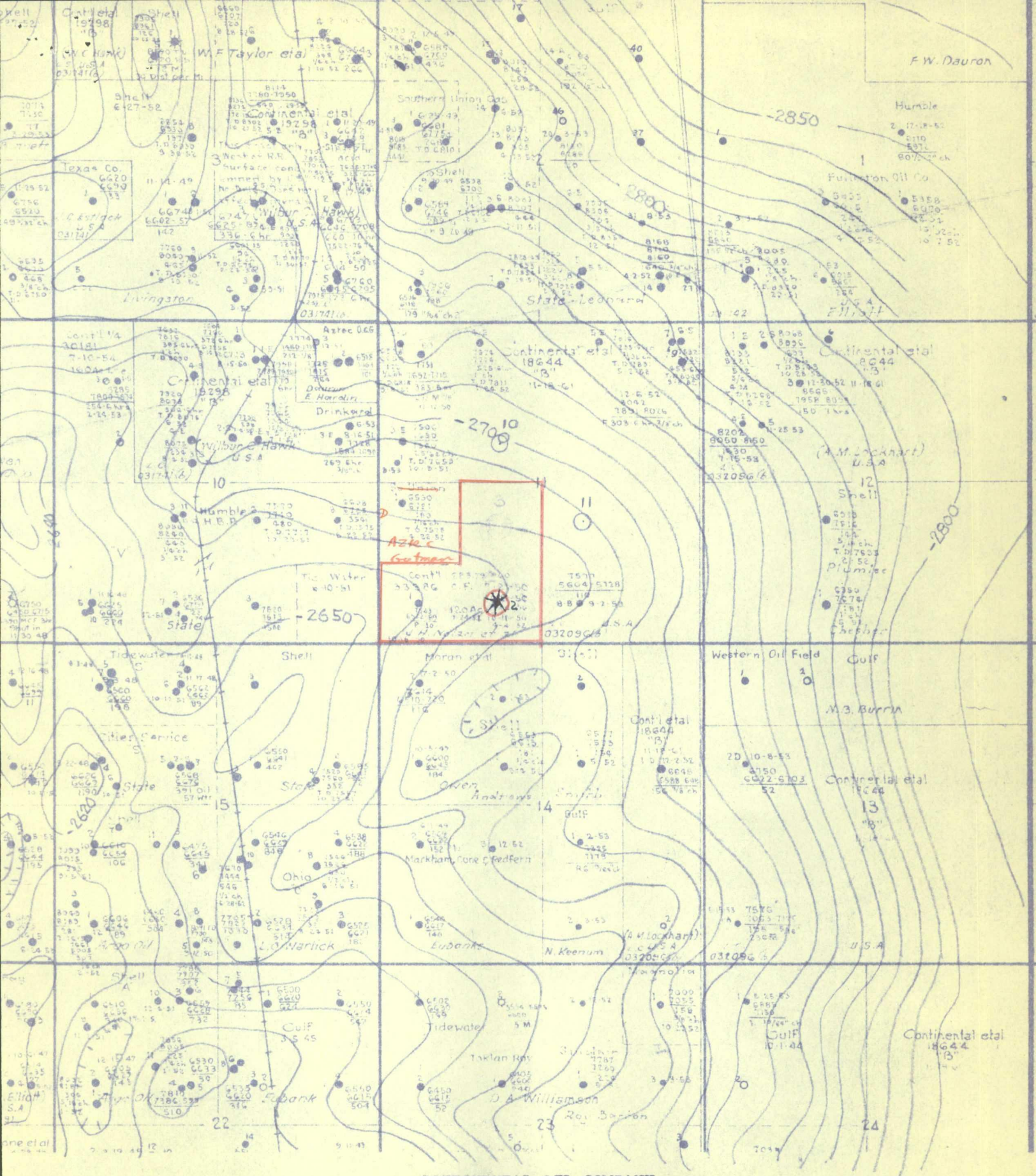
CONTINENTAL OIL COMPANY CONTOURED ON TOP OF THE TUBB C. I. 10' Scale 1" = 2000' T21S - R37E, Lea County, New Mexico Geological Section - Hobbs, N. Mex. Aug. 31, 1954
