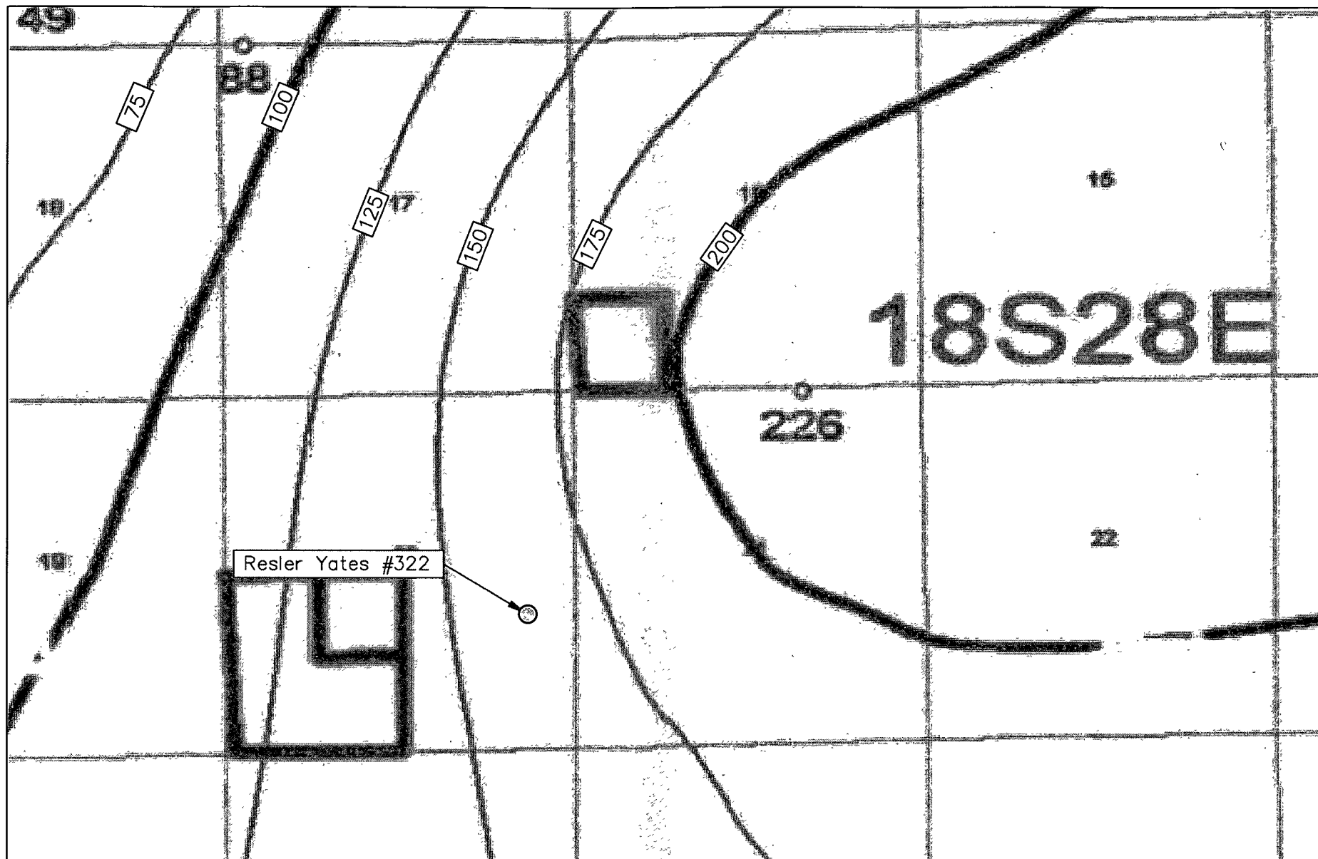
Figure 3 Groundwater Gradient Map Sandlot Energy Resler Yates #322
