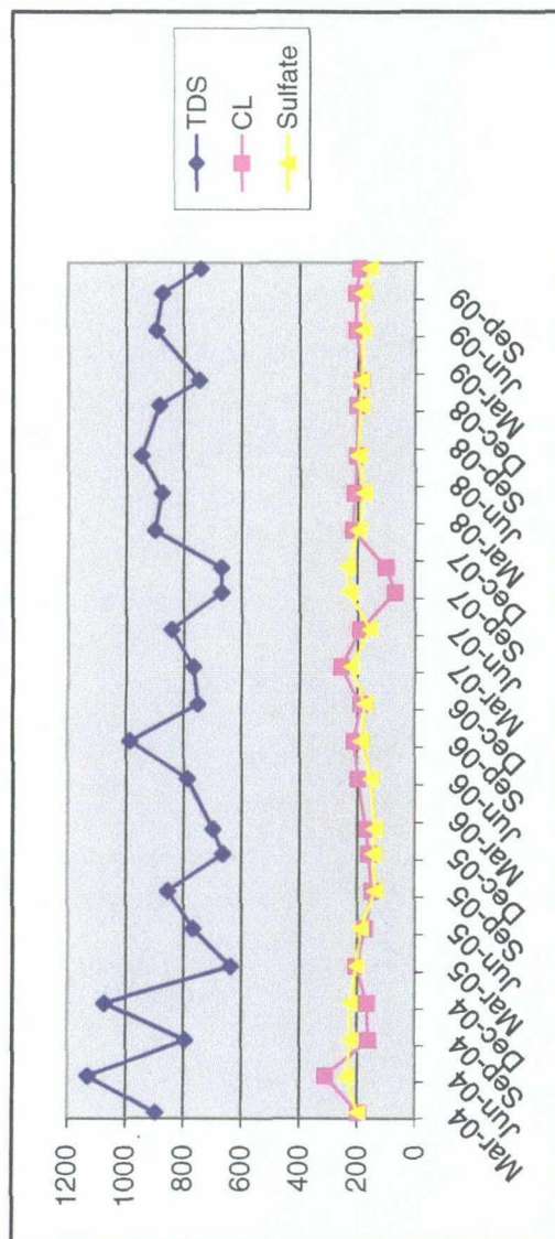
Graph 6 Rice Operating Company MW-5 Justis H-2 Lea County, New Mexico
