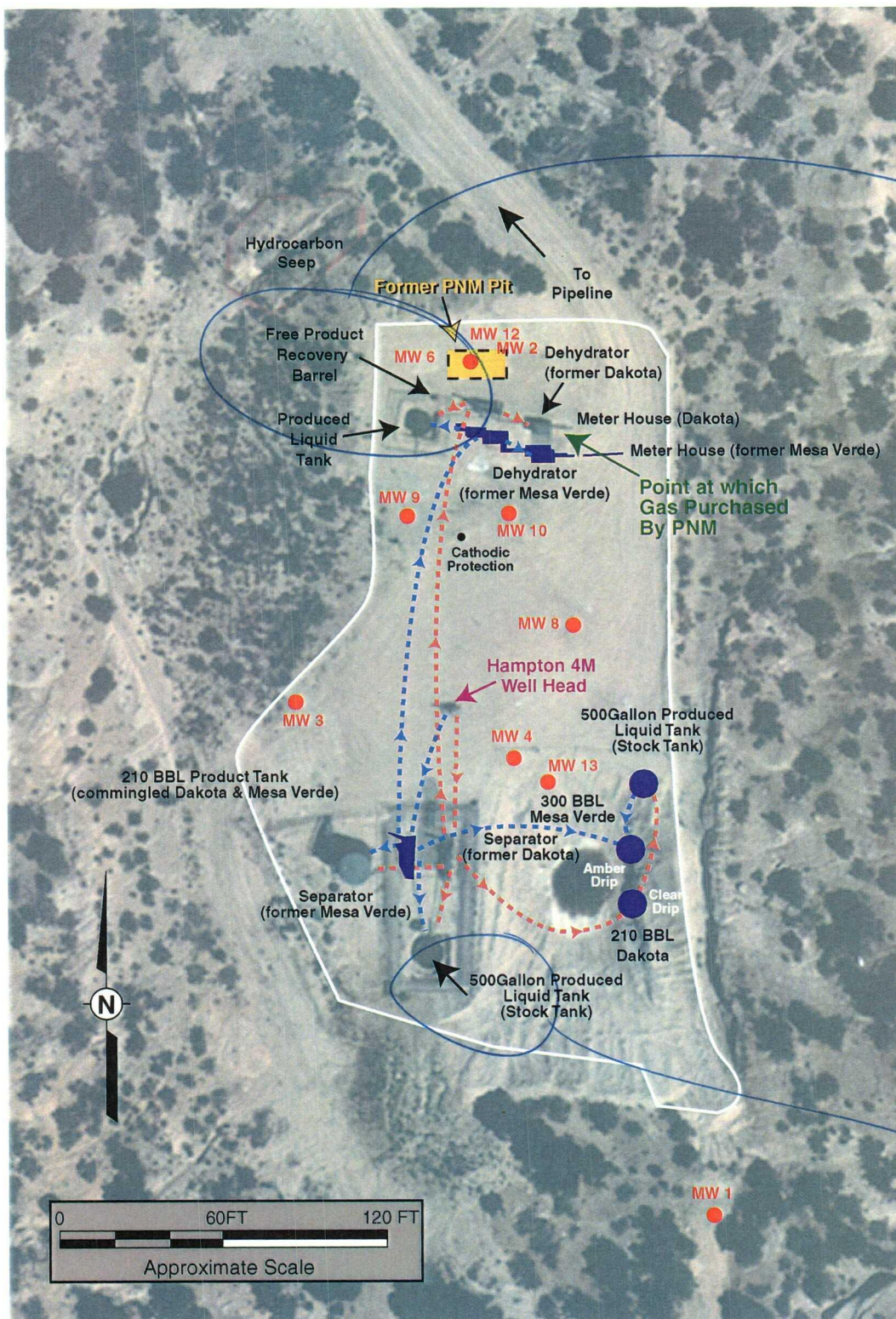
Hampton 4M Site Map Dual Production Operations (<1998)
