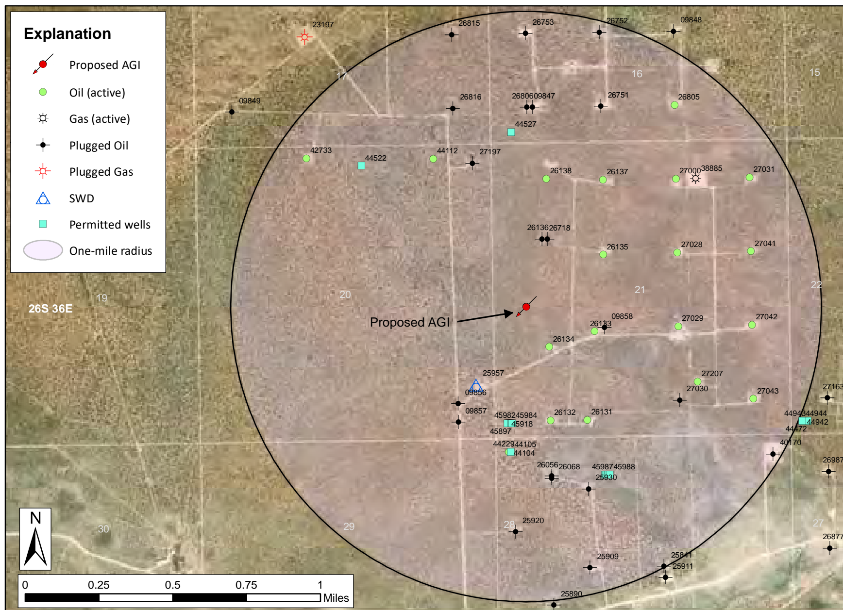
Figure A-1. All wells located within a one-mile radius of the proposed Salt Creek AGI #1. Wells are labeled with the final five numerals of their API 30-025-XXXXX.
