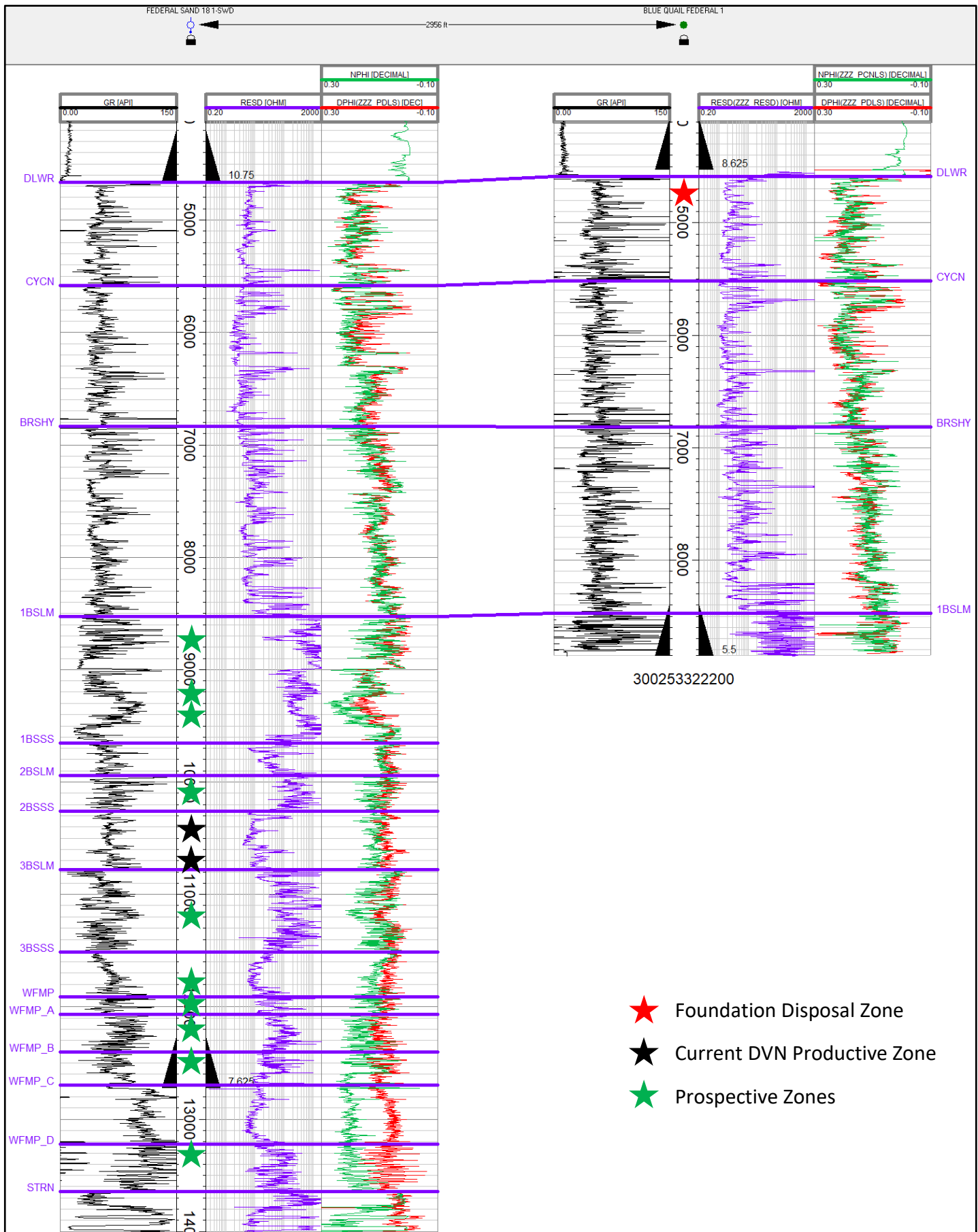
Devon Exhibit B-3 – Two well cross section A-A' shows Devon Energy's current productive and prospective zones in the Federal Sand 18 1-SWD (30-025-25017) in comparison to the proposed Blue Quail Federal 1 (30-025-33222) disposal zone.
