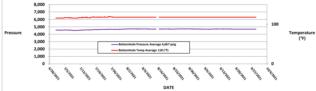
FIGURE 5: MONUMENT AGI D #2 BOTTOM HOLE PRESSURE AND TEMPERATURE
