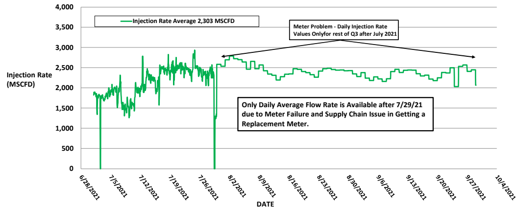
FIGURE 1: MONUMENT AGI D #2 INJECTION RATES WHILE OPERATING
