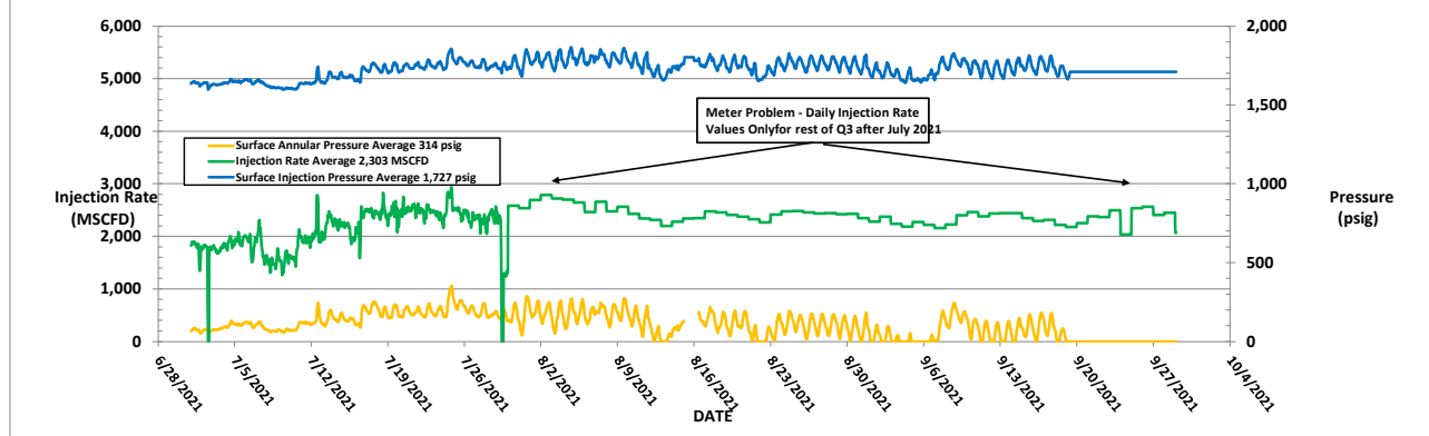
FIGURE 2: MONUMENT AGI D #2 SURFACE INJECTION PRESSURE, ANNULAR PRESSURE AND INJECTION RATE
