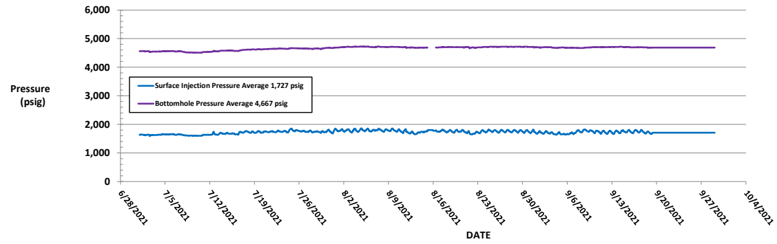
FIGURE 4: MONUMENT AGI D #2 SURFACE INJECTION PRESSURE AND BOTTOM HOLE PRESSURE
