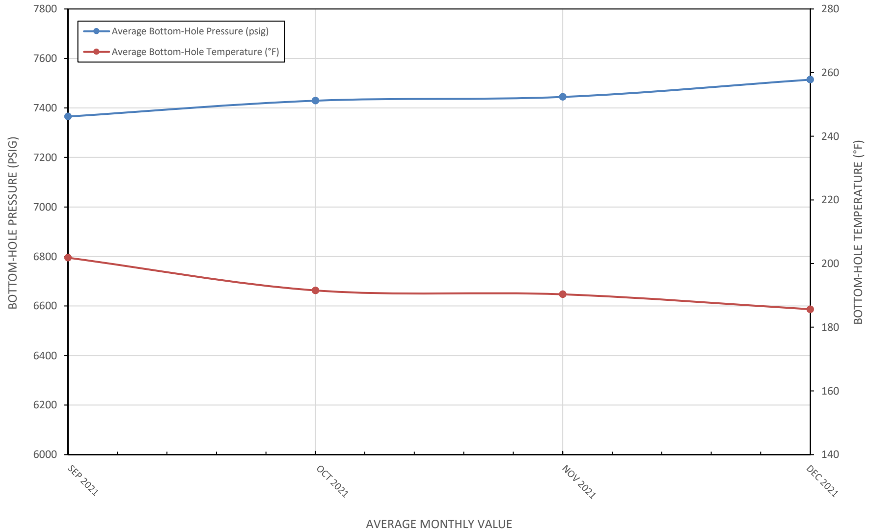
FIGURE 2. INDEPENDENCE AGI #1 SUMMARY OF BOTTOM-HOLE INJECTION DATA
