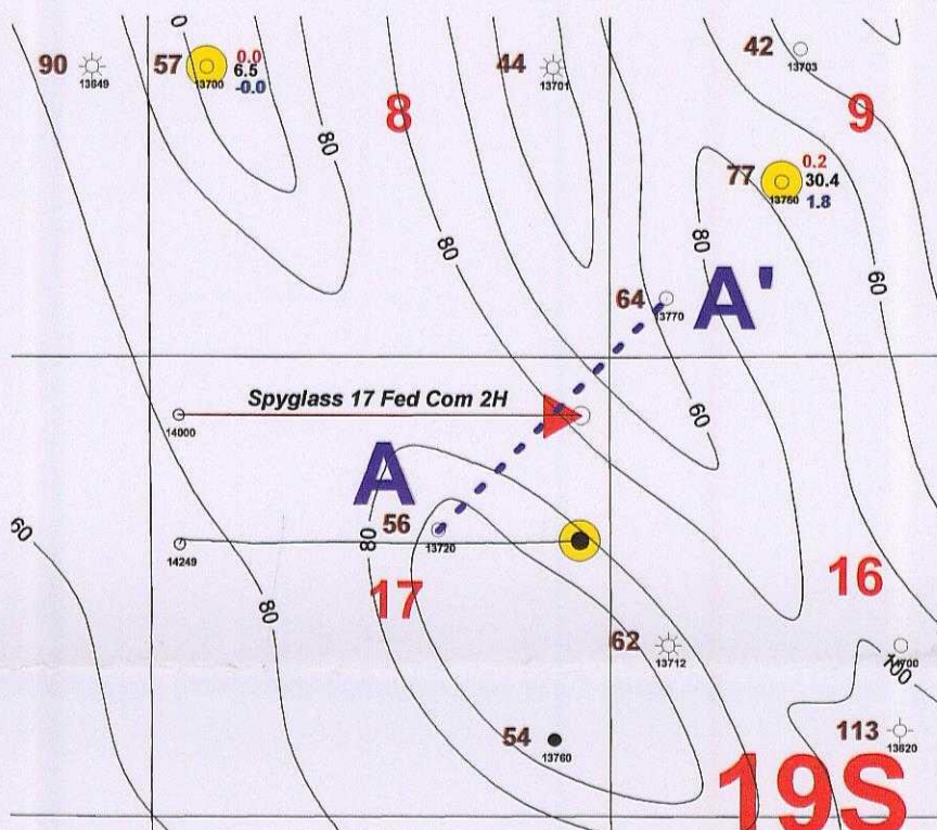
Gross Isopach 2nd BSPG "C" Sd (C.I. 20)
