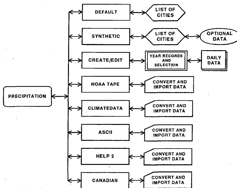
Figure 8. Precipitation Options
