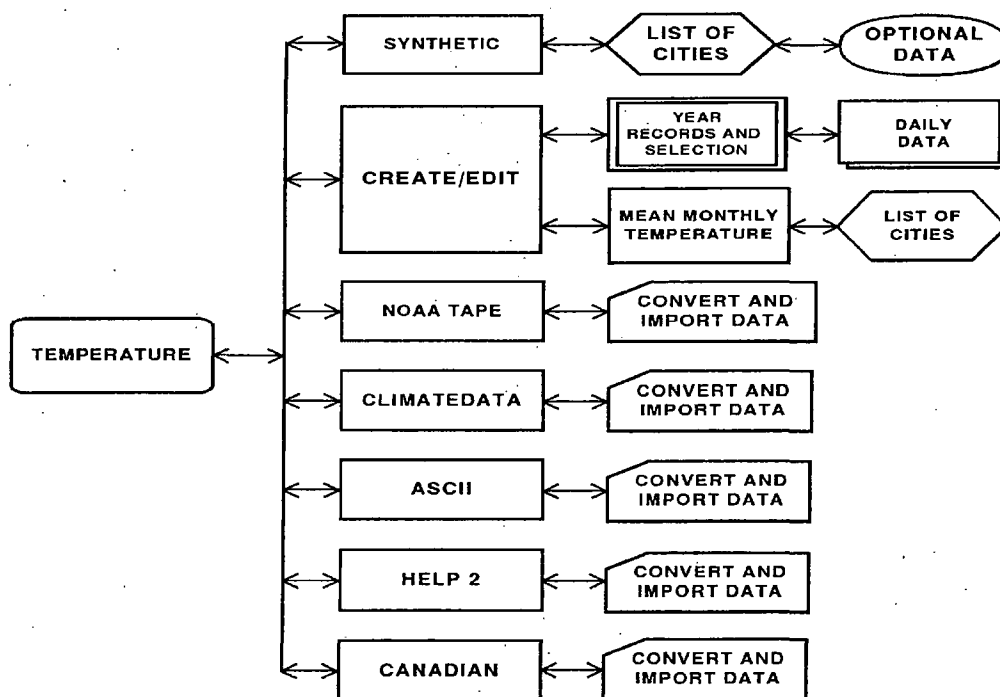
Figure 9. Temperature Options
