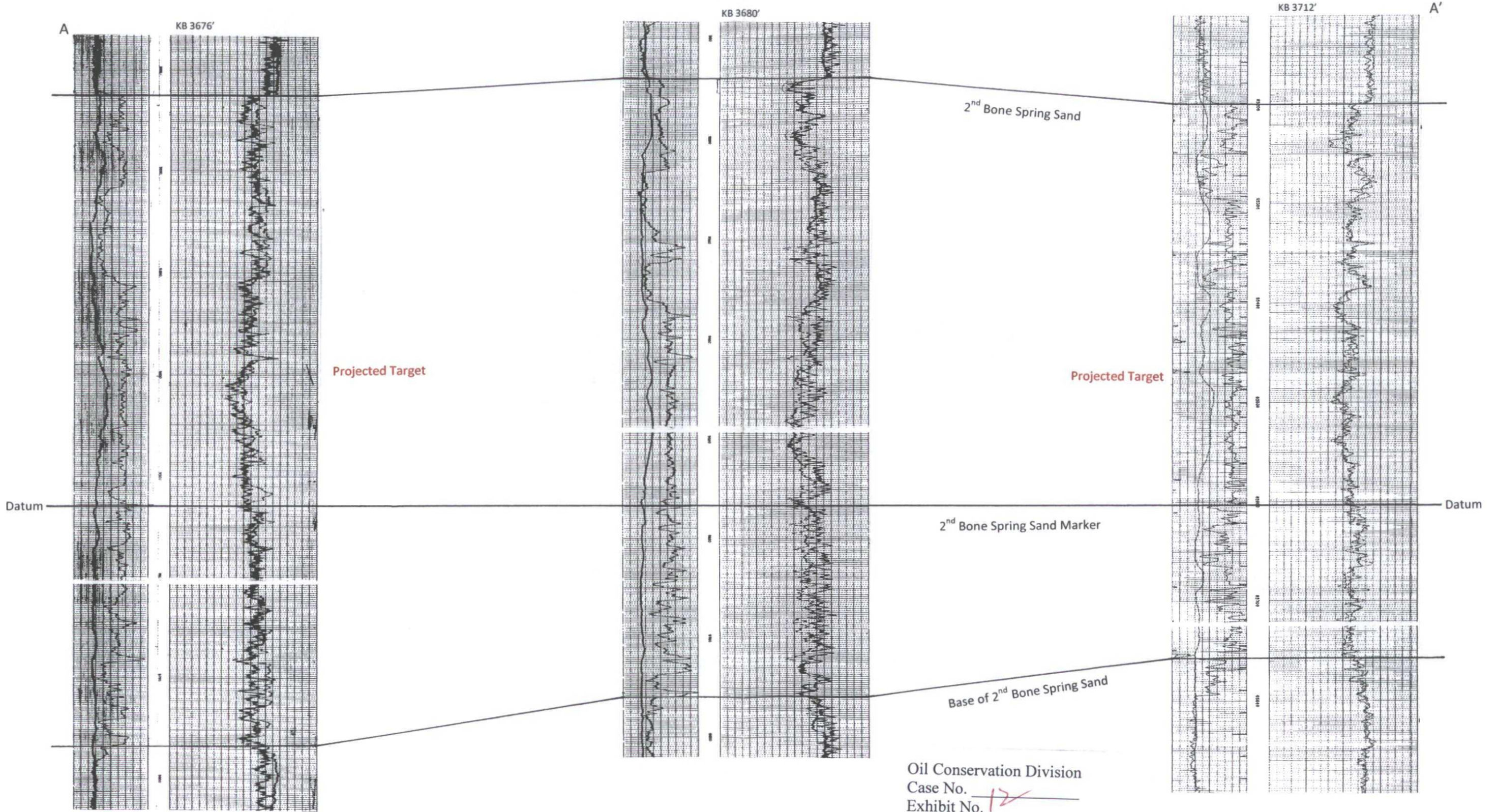
STRATIGRAPHIC CROSS-SECTION A-A' MARSHALL & WINSTON, INC.
