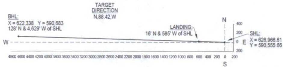
HORIZONTAL PROJECTION
