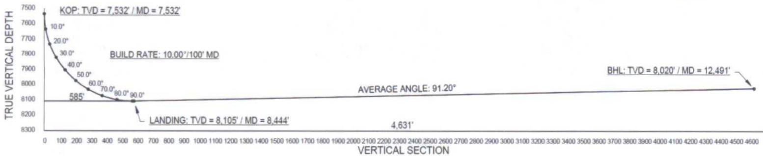
VERTICAL PROJECTION
