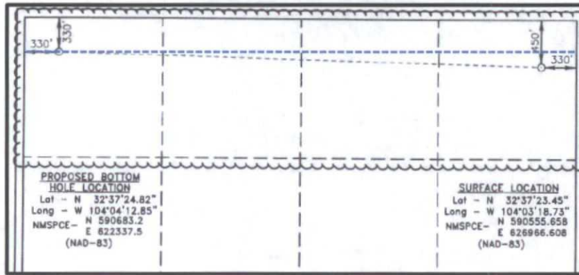
HORIZONTAL PROJECTION
