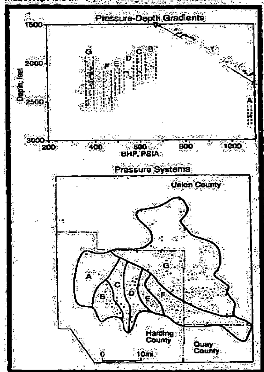
Figure 4. Pressure-depth gradients and pressure systems in Tubb reservoir, Brava dome field. Based on 119 original shut-in bottom-hole pressures submitted by Amoco to the New Mexico Oil Conservation Division.
