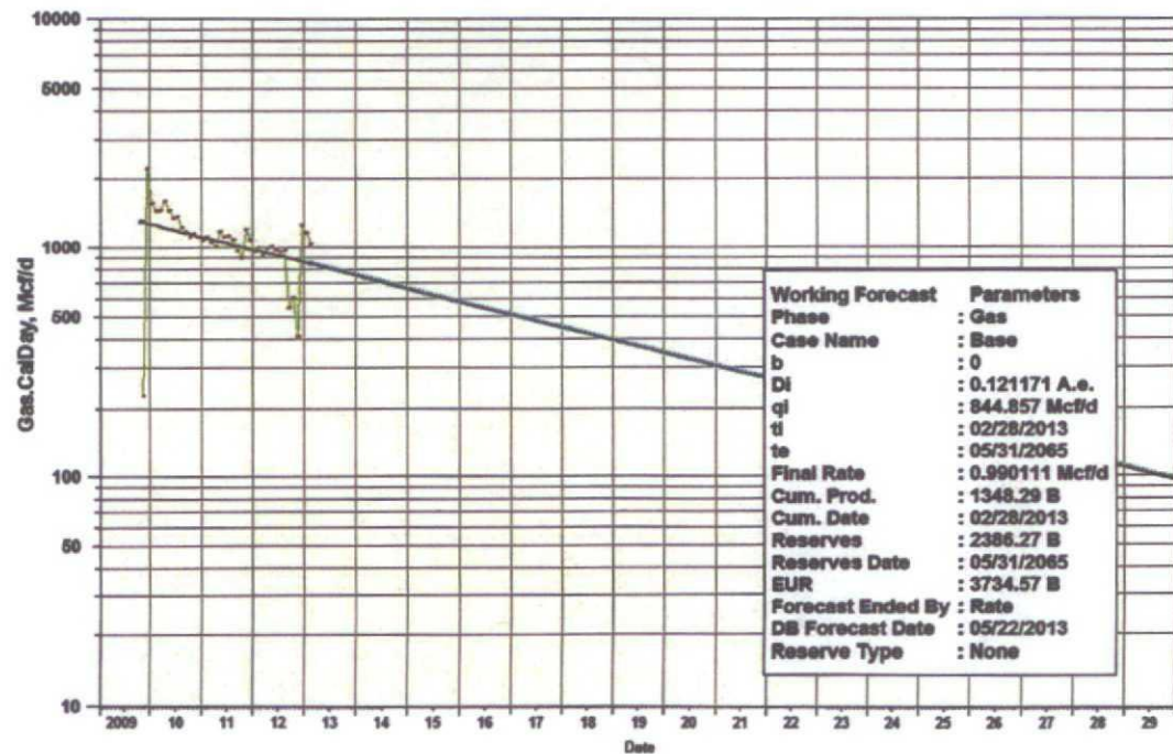
BRAVO_DOME_CARBON_DIOXIDE_GAS_UNIT_#121A | 30021201110000:CO2
