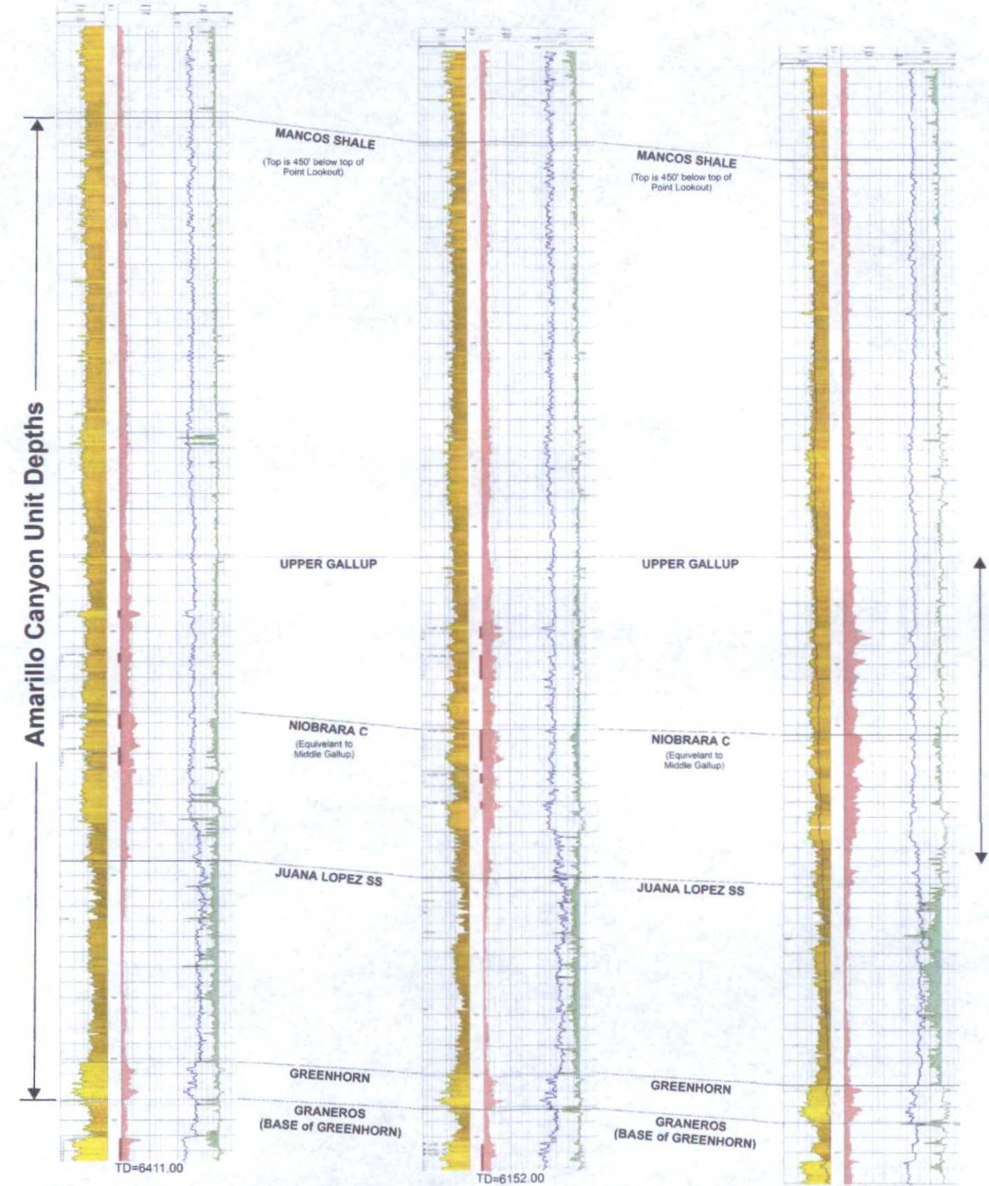
Amarillo Canyon Federal Unit Stratigraphic Cross Section A – A' Datum – Top Upper Gallup
