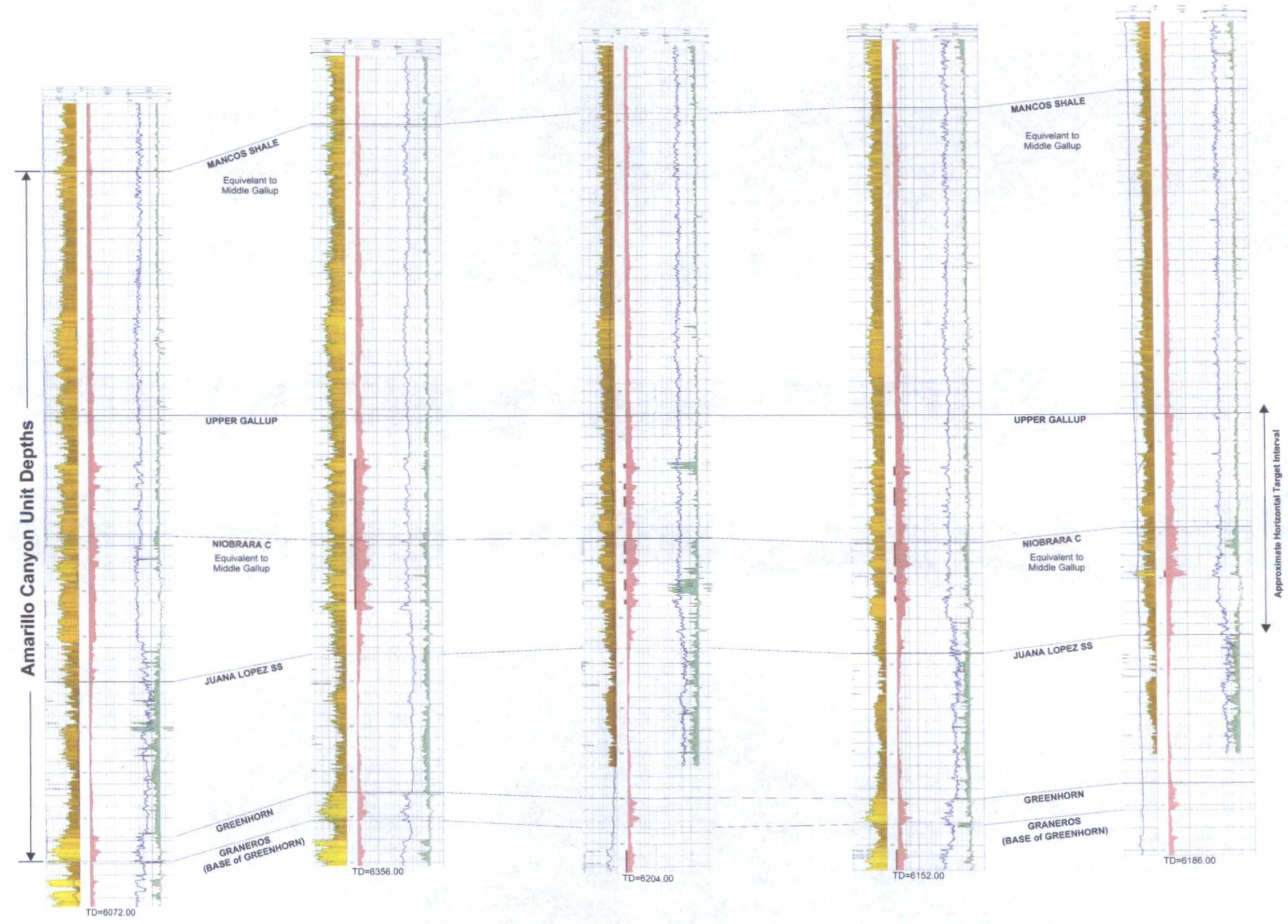
Amarillo Canyon Federal Unit Stratigraphic Cross Section B – B' Datum – Top Upper Gallup
