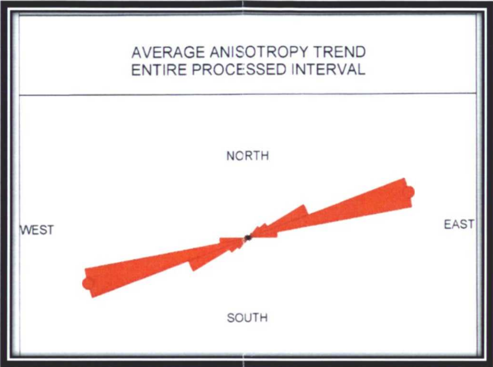
Maximum Principal Stress = N75°E
