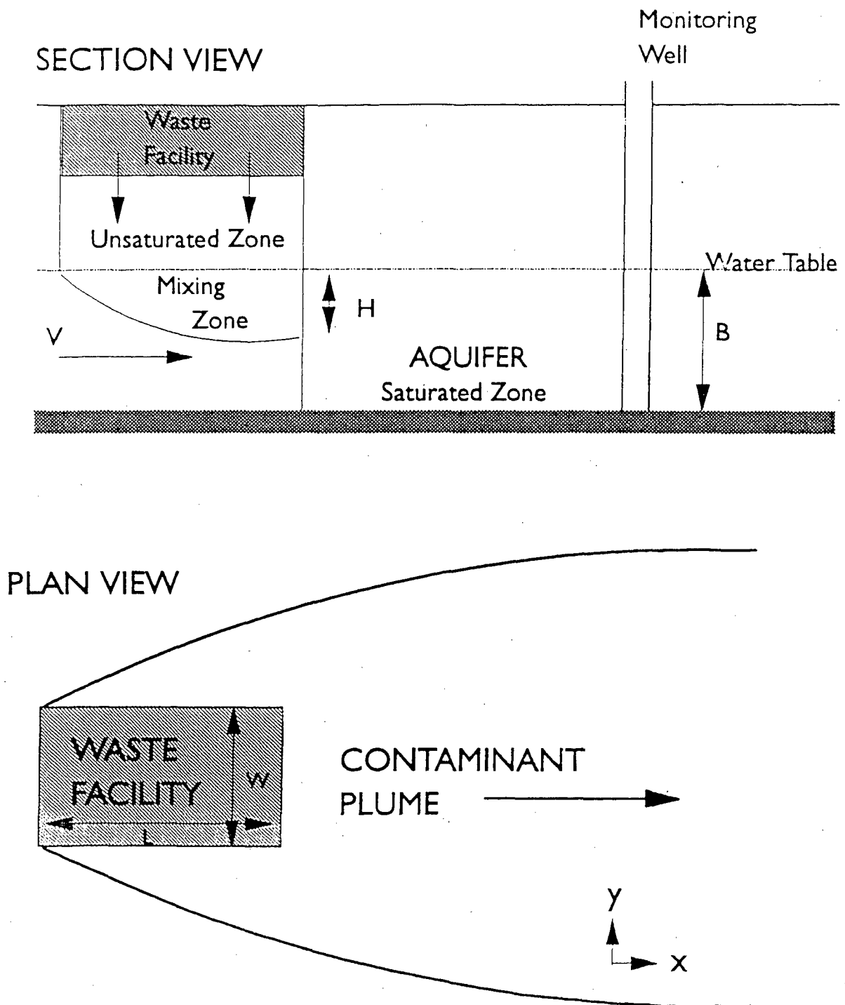
Figure 2.2 Waste facility schematic and MULTIMED geometry (after Salhotra et al., 1990).
