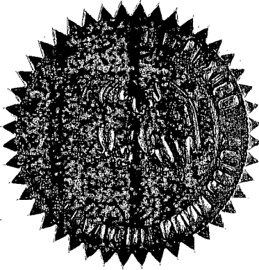
SEAL
