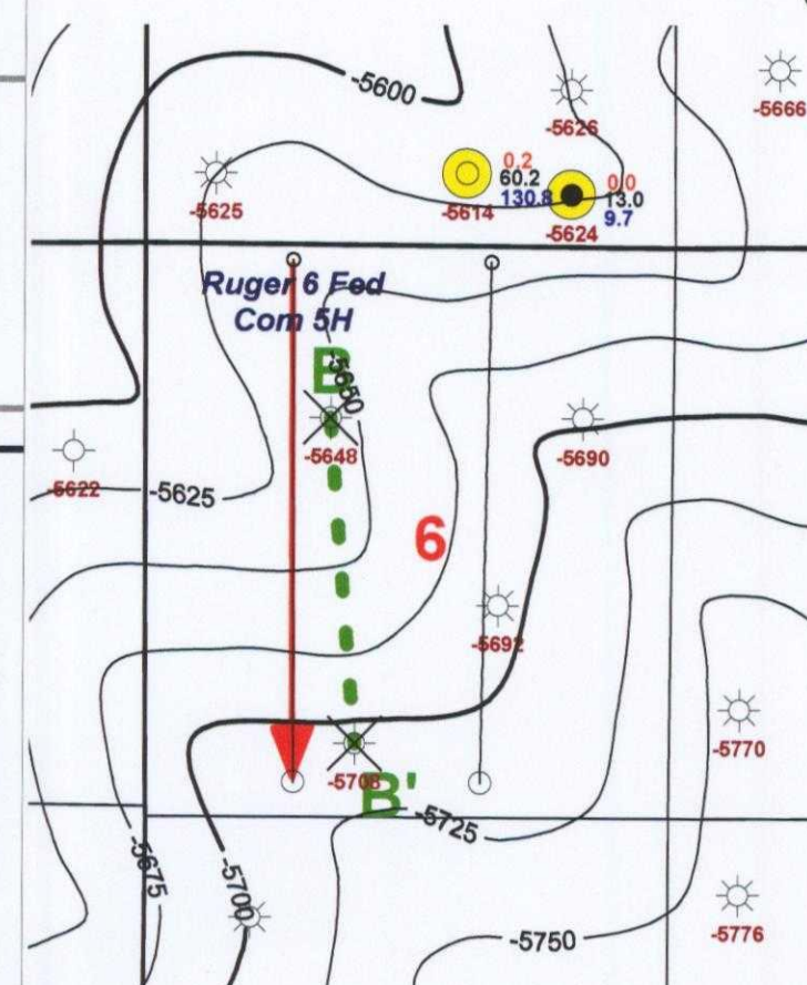
Structure Map on 3rd BSPG Brn Sh Mkr (C.I.25')
