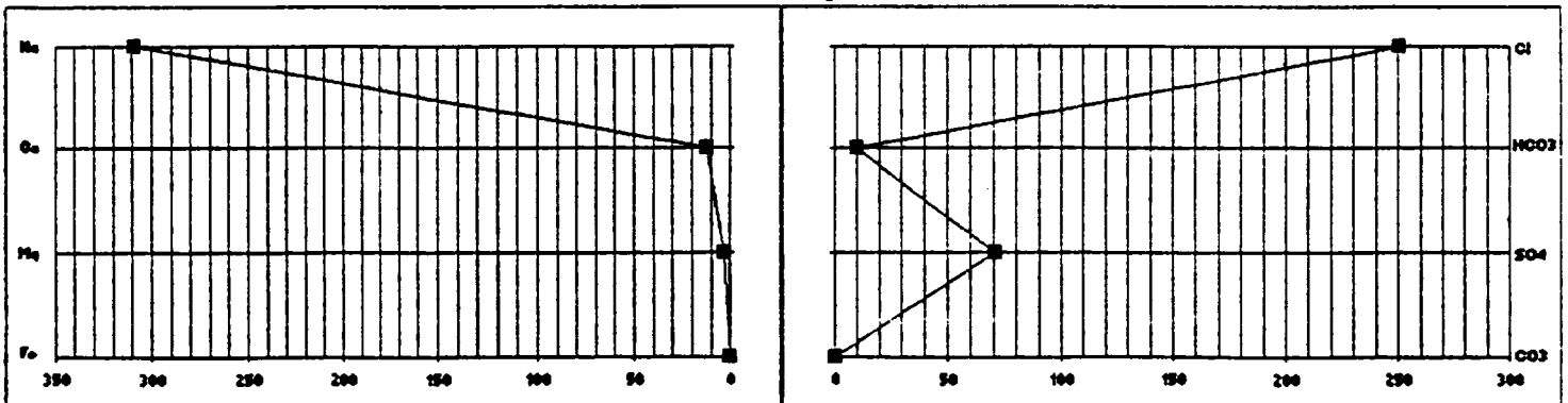
Stiff Diagram
