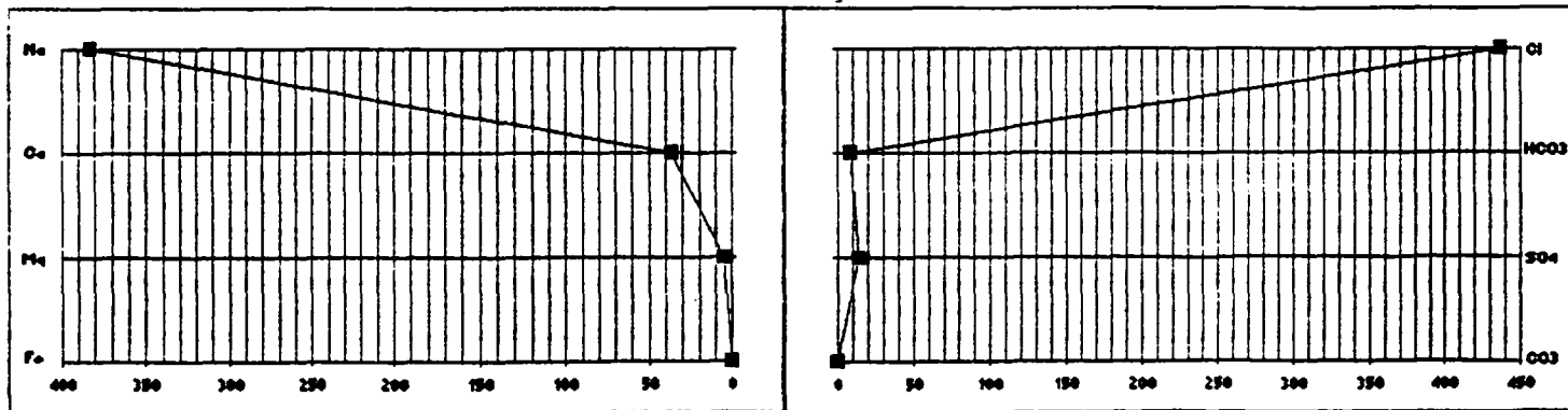
Stiff Diagram
