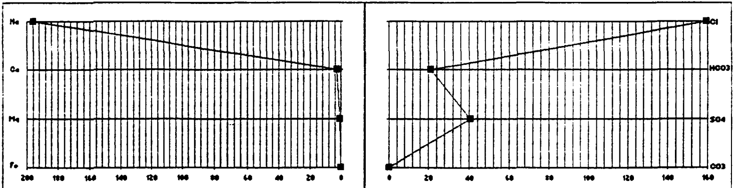
Stiff Diagram
