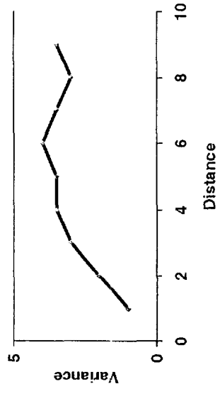
Variogram (Strike)
