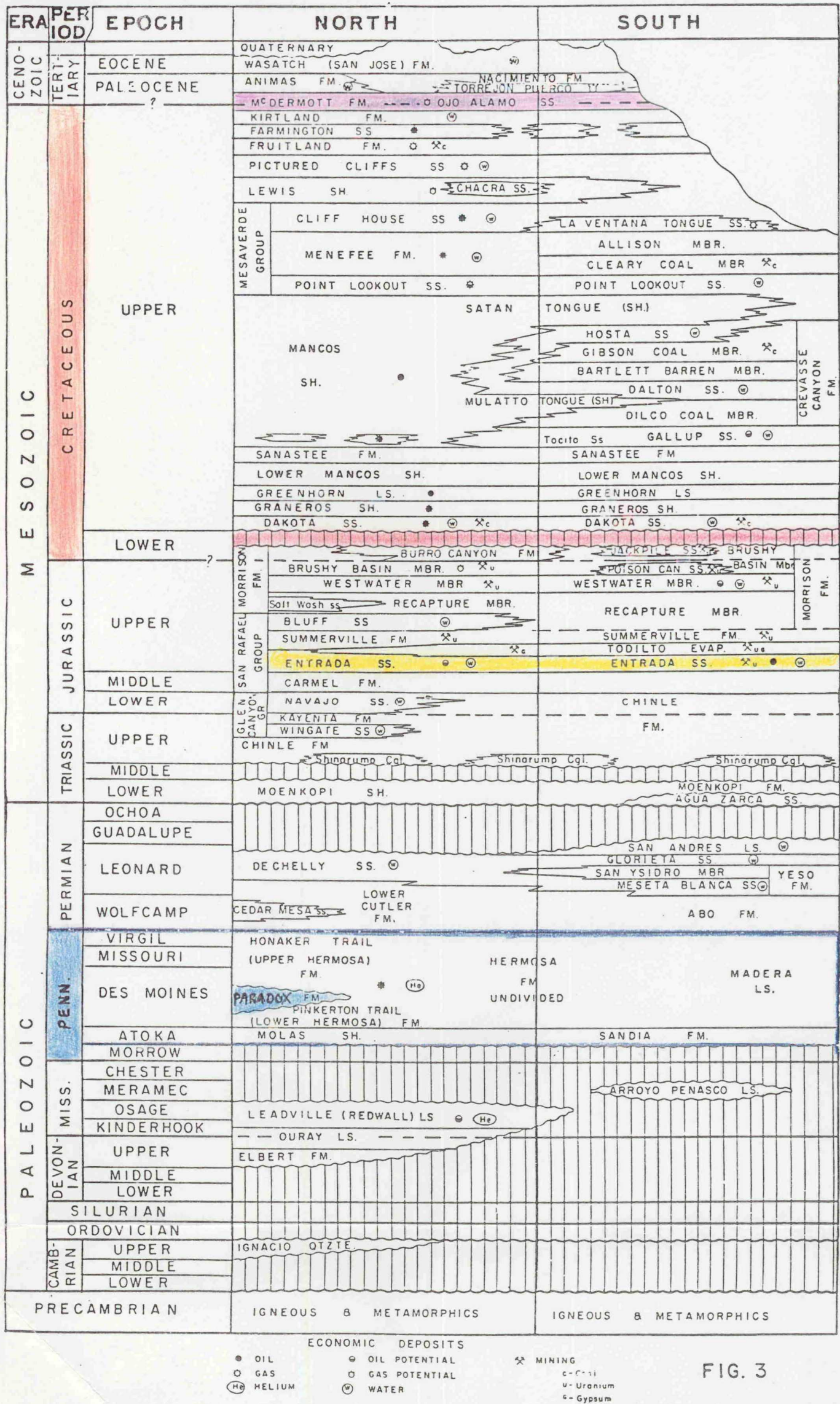
FIG. 3.—Stratigraphic correlation chart of San Juan basin showing economic deposits of current interest.
