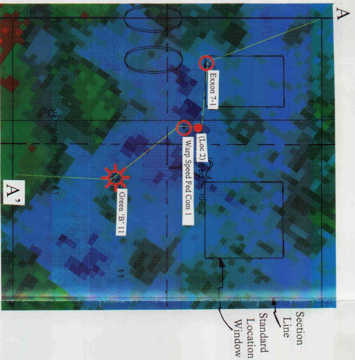
Atoka to Barnett Isochron
