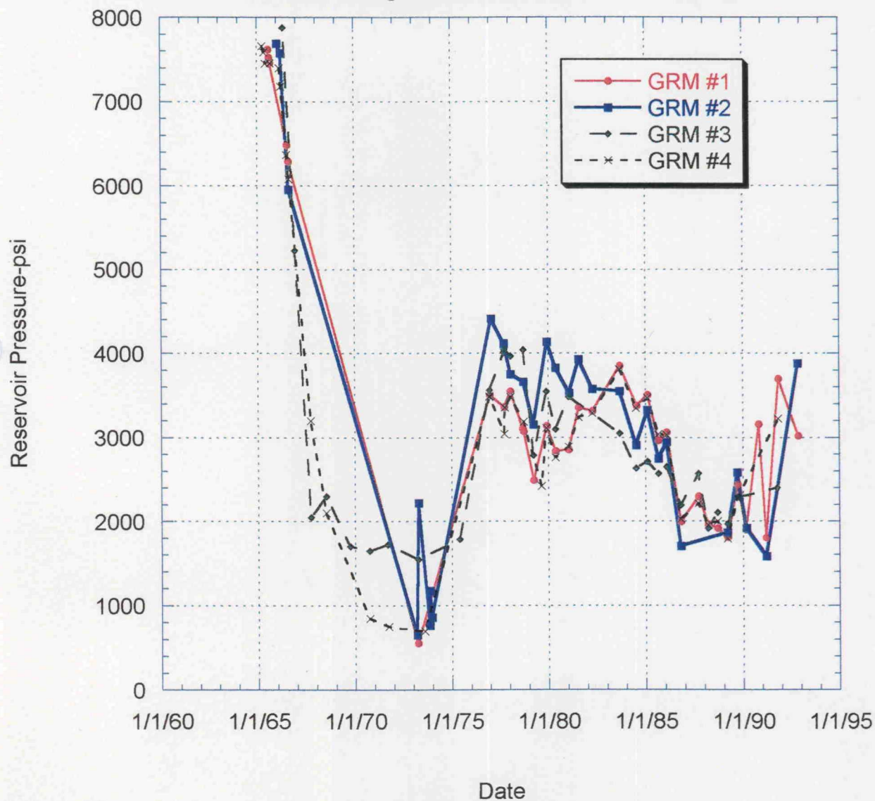
GRM Unit Morrow Gas Storage Unit Reservoir Pressure vs. Time
