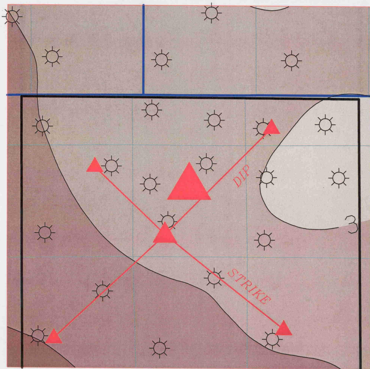
San Juan 28-5 Unit #201S NW15 - T28N- -R5W Pictured Cliffs Structure CI = 50''
