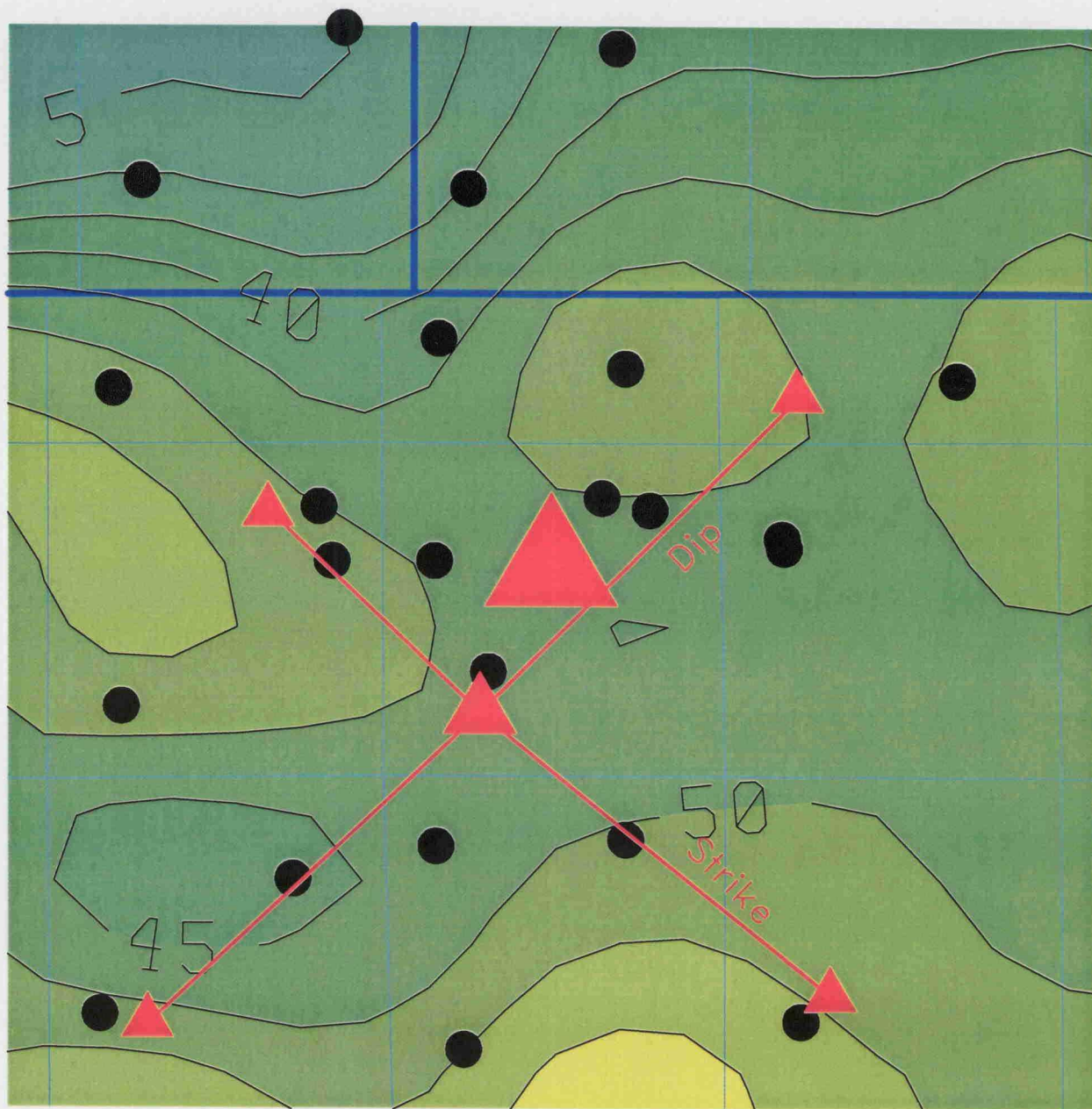
San Juan 28-5 Unit #201S NW15 - T28N - R6W Net Coal - CI=5'
