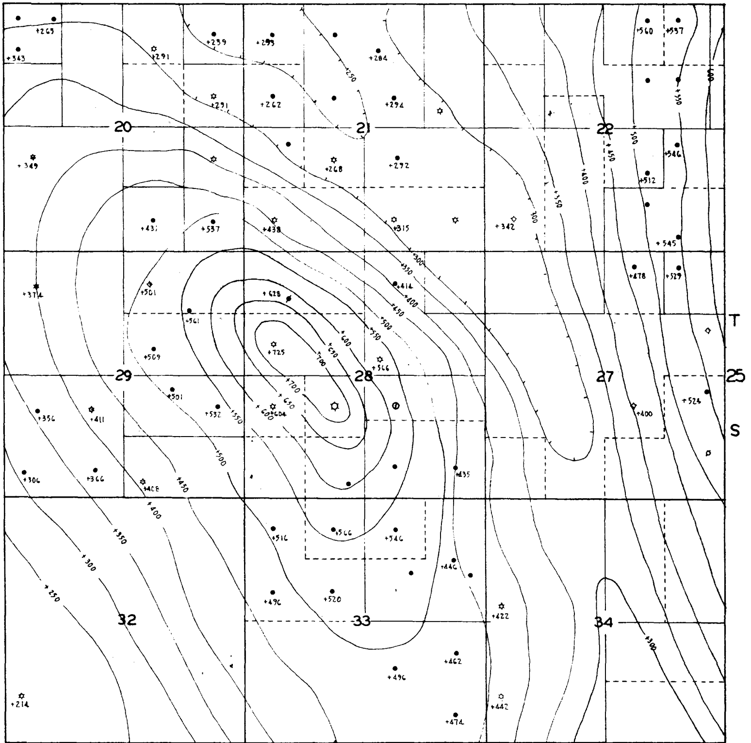
Crosbie (Devonian) Field Lea County, New Mexico Structure Map - Top of Yates Sand
