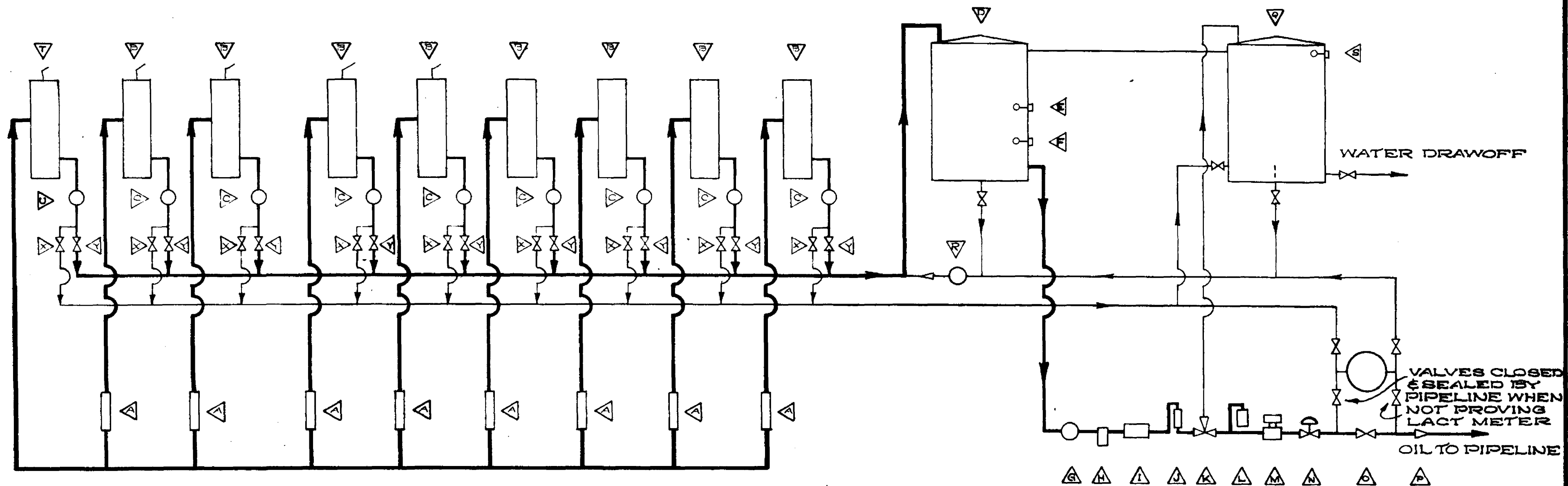
PAN AMERICAN PETROLEUM CORPORATION SCHEMATIC FLOW DRAWING - PROPOSED STORAGE SYSTEM V - CENTRAL BATTERY + LACT UNIT TO SERVE STATE LEASES - EMPIRE ABO POOL - EDDY COUNTY - NEW MEXICO
