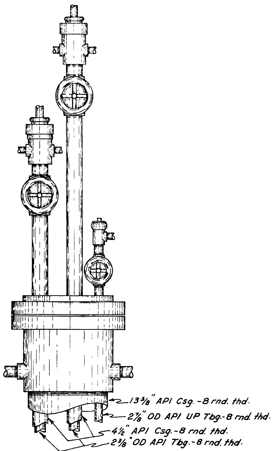
Landing Mandrels
