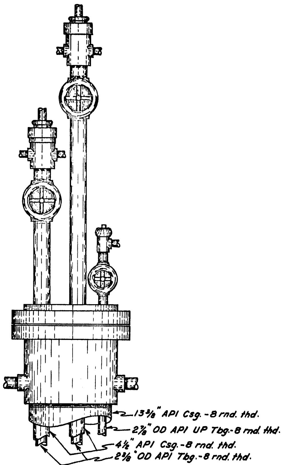
Landing Mandrels
