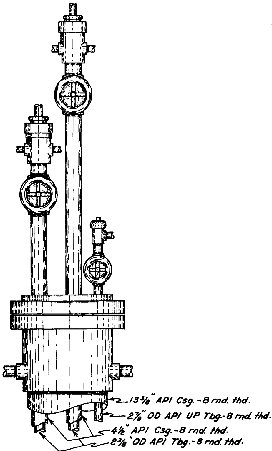
Landing Mandrels
