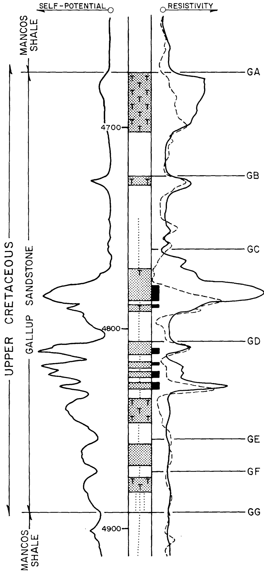
LEGEND Microlog Net Pay TYPE LOG BISTI FIELD GALLUP SANDSTONE SCALE : 1" = 30'
