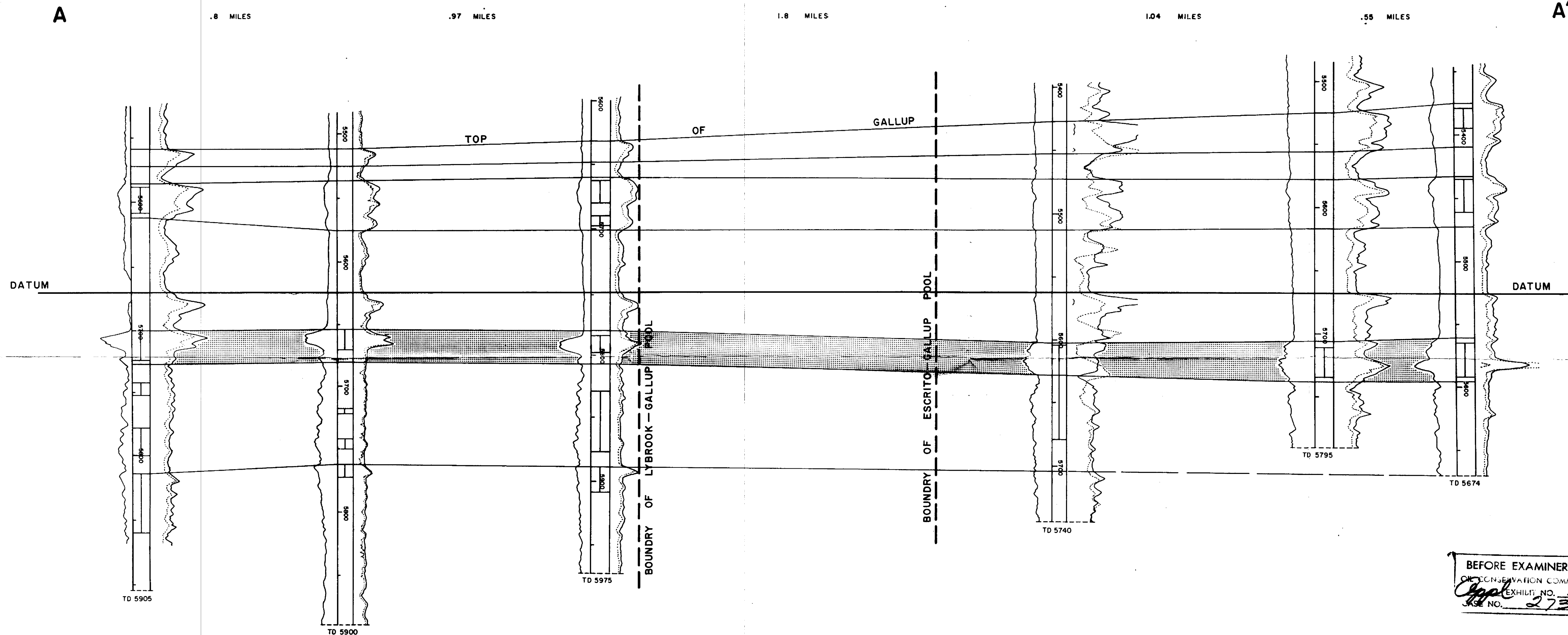
SOUTH-NORTH CROSS SECTION A-A' LYBROOK-GALLUP AND ESCRITO-GALLUP OIL POOLS RIO ARRIBA CO., NEW MEXICO
